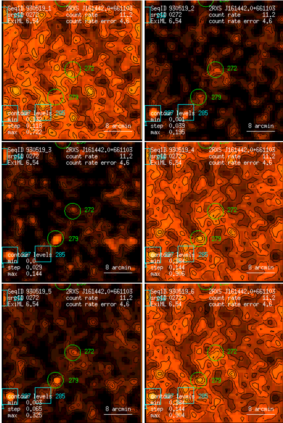
Figure 272: RASS 930519: detection 0272: band rate images, Gaussian filter: (1) PSPC channels 11 – 41, (2) 52 – 90, (3) 91 – 201, (4) 11 – 235, (5) 52 – 201, (6) 11 – 201. Broad band rates in counts/ks. Band rate contour levels in counts/ks/arcmin 2 .
