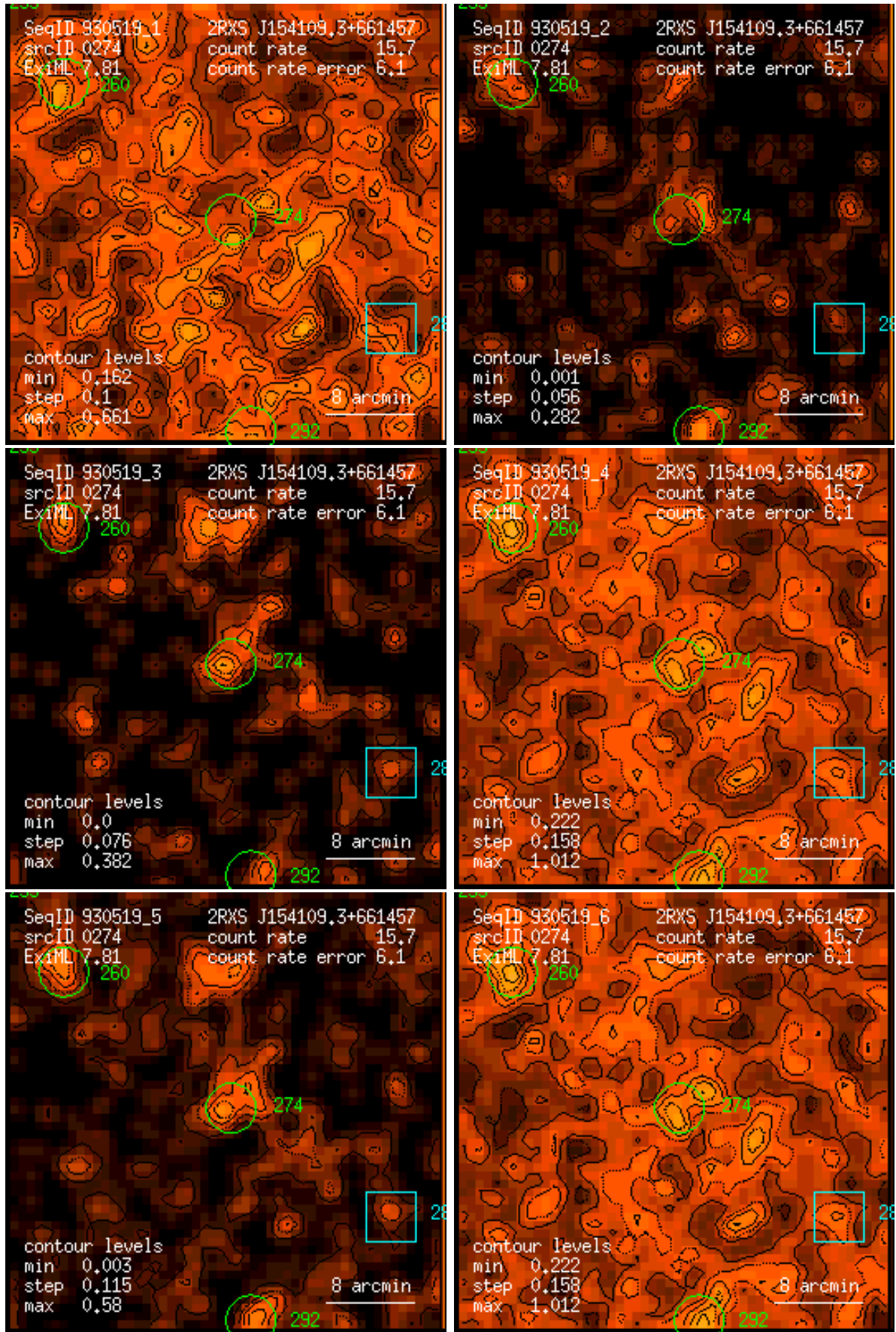
Figure 274: RASS 930519: detection 0274: band rate images, Gaussian filter: (1) PSPC channels 11 – 41, (2) 52 – 90, (3) 91 – 201, (4) 11 – 235, (5) 52 – 201, (6) 11 – 201. Broad band rates in counts/ks. Band rate contour levels in counts/ks/arcmin 2 .
