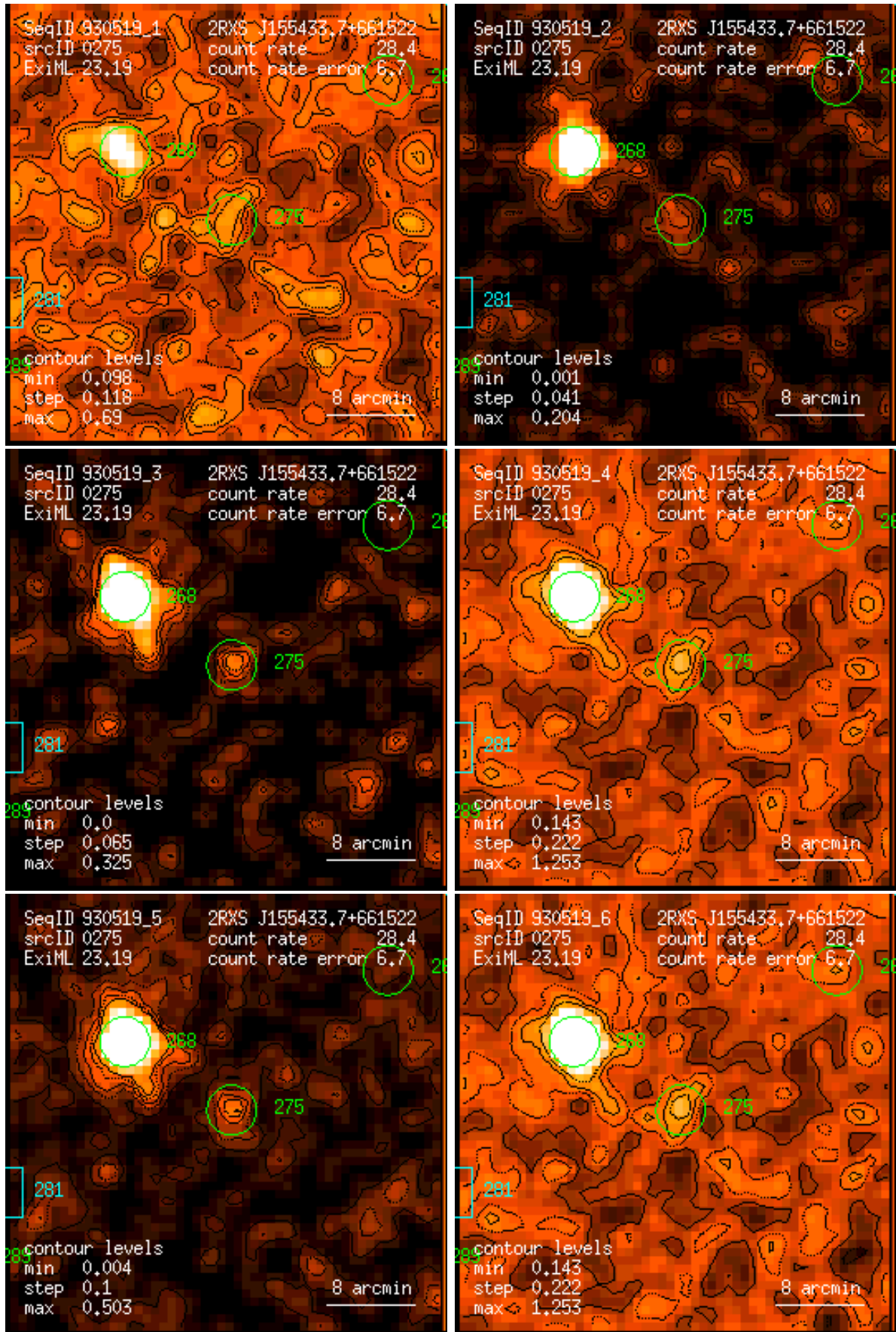
Figure 275: RASS 930519: detection 0275: band rate images, Gaussian filter: (1) PSPC channels 11 – 41, (2) 52 – 90, (3) 91 – 201, (4) 11 – 235, (5) 52 – 201, (6) 11 – 201. Broad band rates in counts/ks. Band rate contour levels in counts/ks/arcmin 2 .
