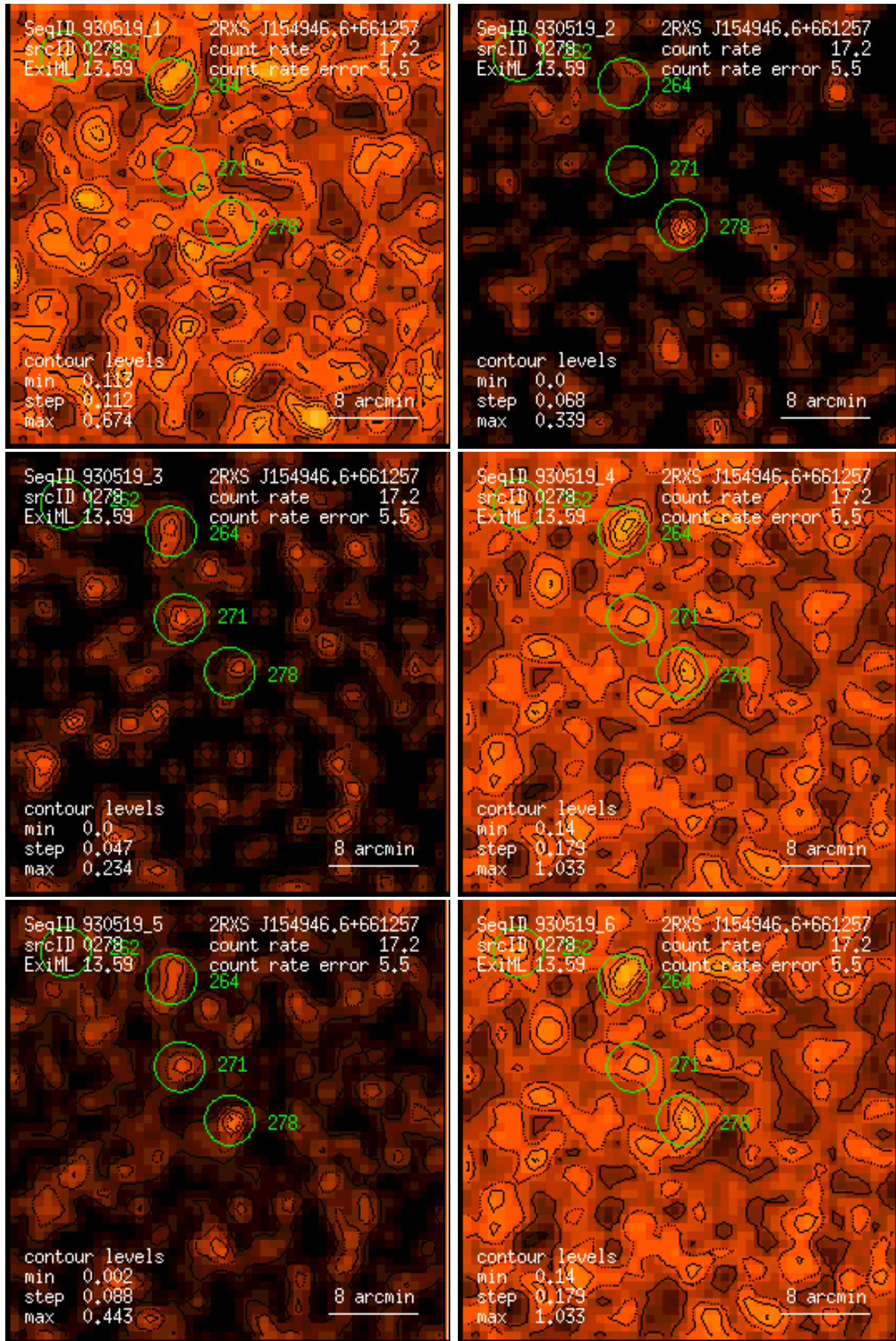
Figure 278: RASS 930519: detection 0278: band rate images, Gaussian filter: (1) PSPC channels 11 – 41, (2) 52 – 90, (3) 91 – 201, (4) 11 – 235, (5) 52 – 201, (6) 11 – 201. Broad band rates in counts/ks. Band rate contour levels in counts/ks/arcmin 2 .
