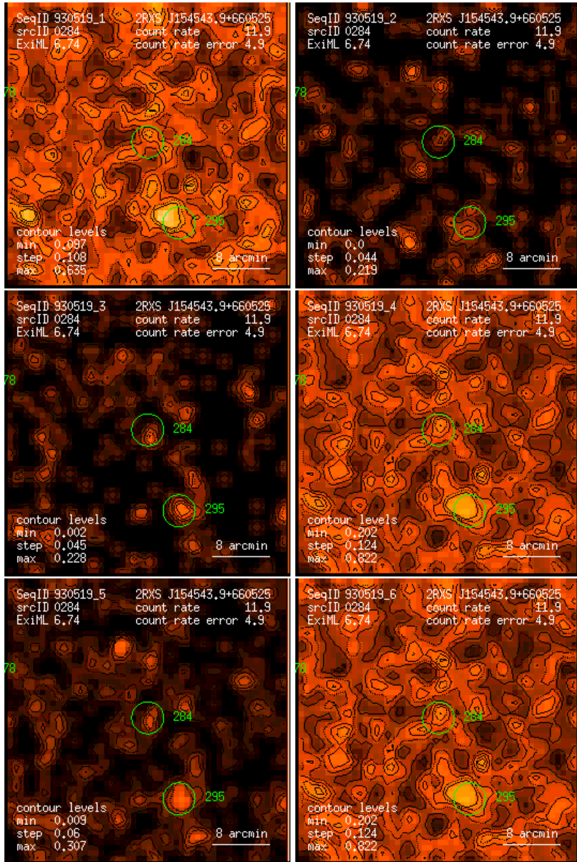
Figure 284: RASS 930519: detection 0284: band rate images, Gaussian filter: (1) PSPC channels 11 – 41, (2) 52 – 90, (3) 91 – 201, (4) 11 – 235, (5) 52 – 201, (6) 11 – 201. Broad band rates in counts/ks. Band rate contour levels in counts/ks/arcmin 2 .
