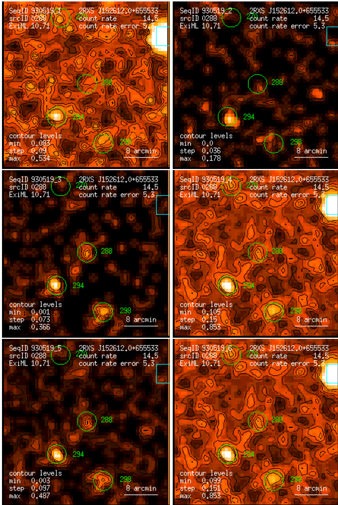
Figure 288: RASS 930519: detection 0288: band rate images, Gaussian filter: (1) PSPC channels 11 – 41, (2) 52 – 90, (3) 91 – 201, (4) 11 – 235, (5) 52 – 201, (6) 11 – 201. Broad band rates in counts/ks. Band rate contour levels in counts/ks/arcmin 2 .
