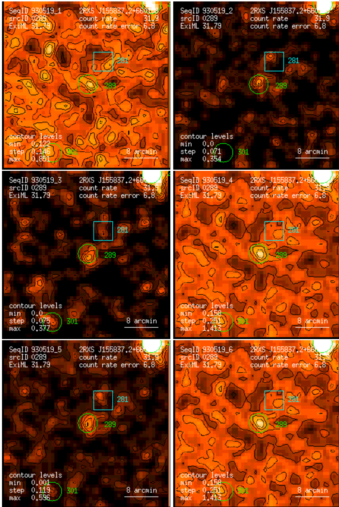
Figure 289: RASS 930519: detection 0289: band rate images, Gaussian filter: (1) PSPC channels 11 – 41, (2) 52 – 90, (3) 91 – 201, (4) 11 – 235, (5) 52 – 201, (6) 11 – 201. Broad band rates in counts/ks. Band rate contour levels in counts/ks/arcmin 2 .
