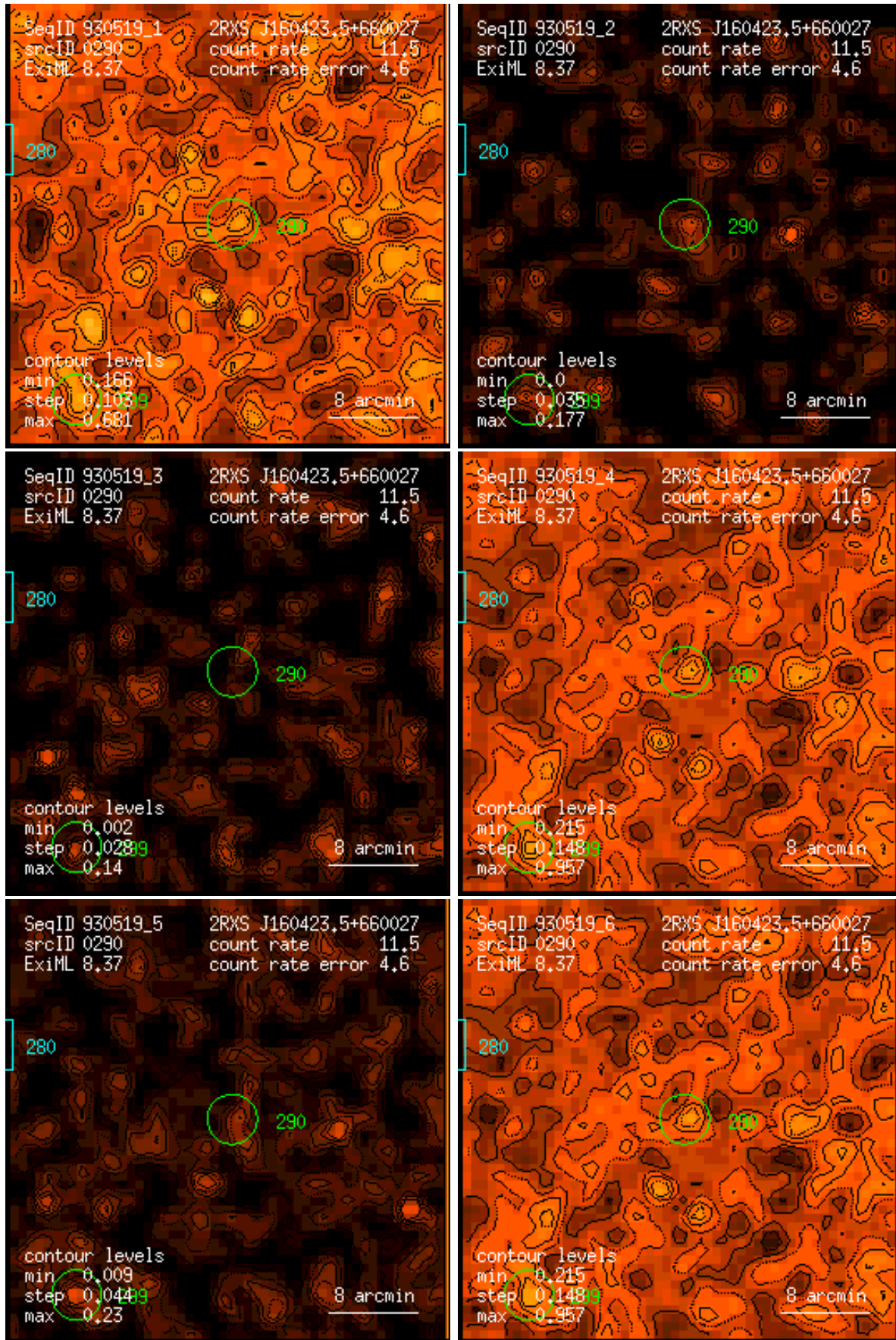
Figure 290: RASS 930519: detection 0290: band rate images, Gaussian filter: (1) PSPC channels 11 – 41, (2) 52 – 90, (3) 91 – 201, (4) 11 – 235, (5) 52 – 201, (6) 11 – 201. Broad band rates in counts/ks. Band rate contour levels in counts/ks/arcmin 2 .
