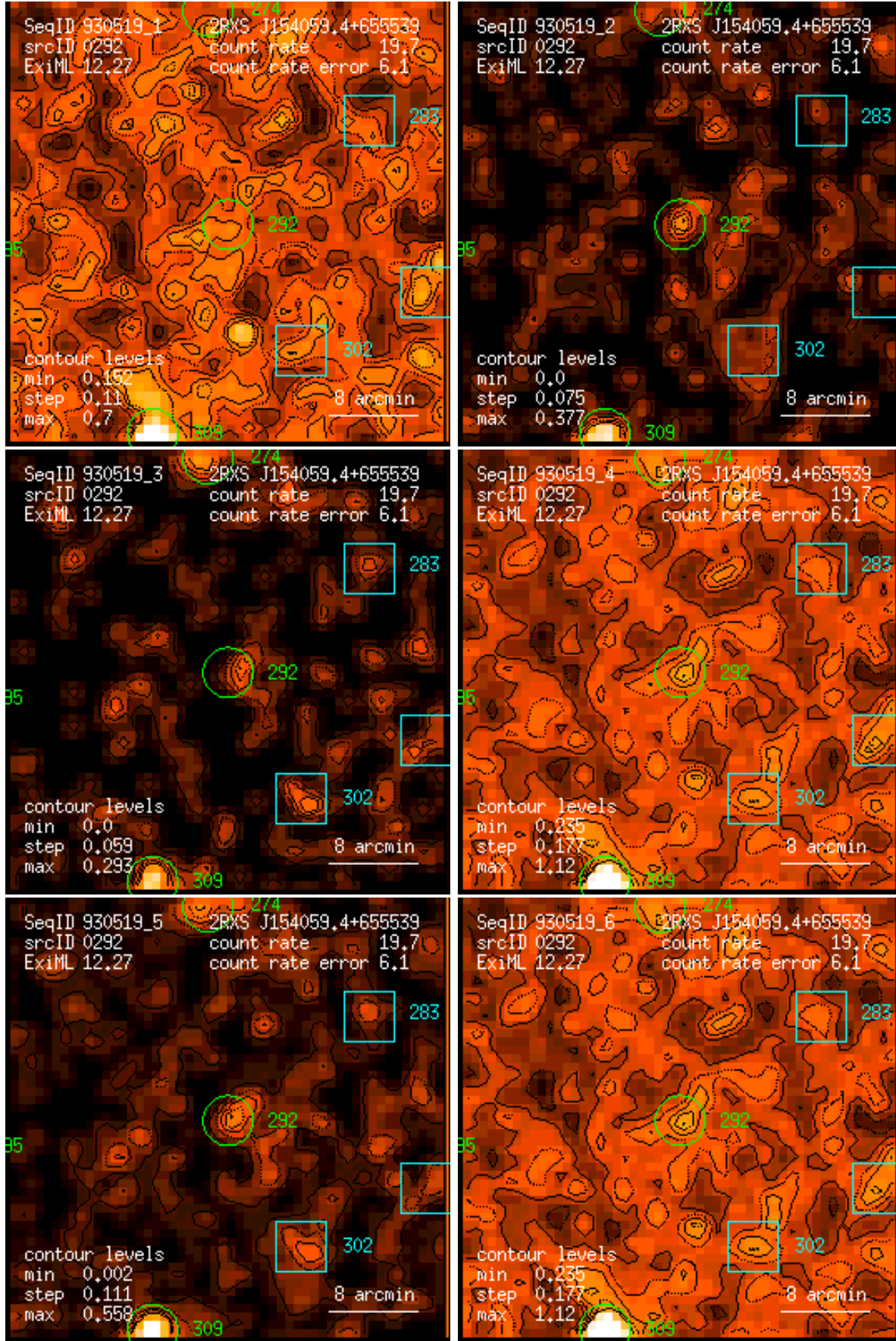
Figure 292: RASS 930519: detection 0292: band rate images, Gaussian filter: (1) PSPC channels 11 – 41, (2) 52 – 90, (3) 91 – 201, (4) 11 – 235, (5) 52 – 201, (6) 11 – 201. Broad band rates in counts/ks. Band rate contour levels in counts/ks/arcmin 2 .
