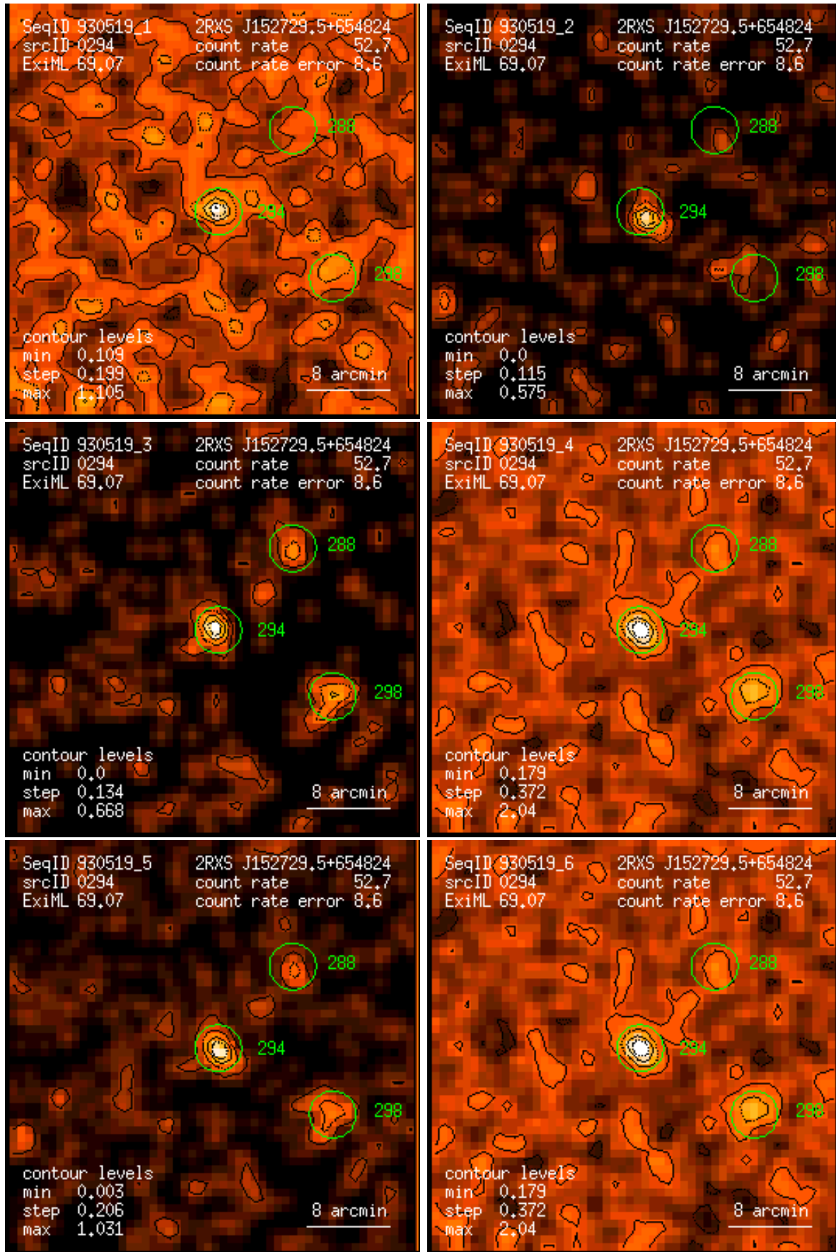
Figure 294: RASS 930519: detection 0294: band rate images, Gaussian filter: (1) PSPC channels 11 – 41, (2) 52 – 90, (3) 91 – 201, (4) 11 – 235, (5) 52 – 201, (6) 11 – 201. Broad band rates in counts/ks. Band rate contour levels in counts/ks/arcmin 2 .
