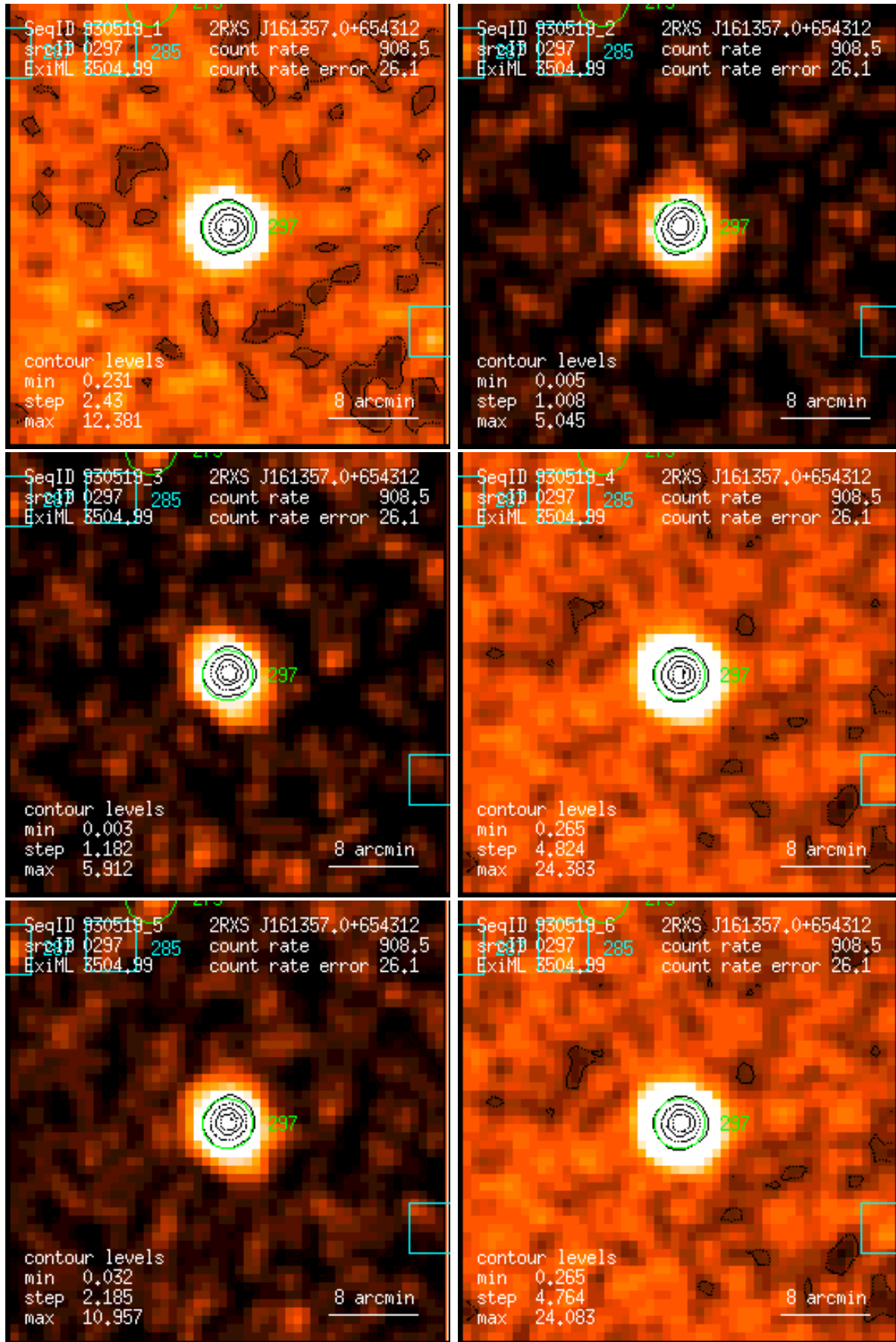
Figure 297: RASS 930519: detection 0297: band rate images, Gaussian filter: (1) PSPC channels 11 – 41, (2) 52 – 90, (3) 91 – 201, (4) 11 – 235, (5) 52 – 201, (6) 11 – 201. Broad band rates in counts/ks. Band rate contour levels in counts/ks/arcmin 2 .
