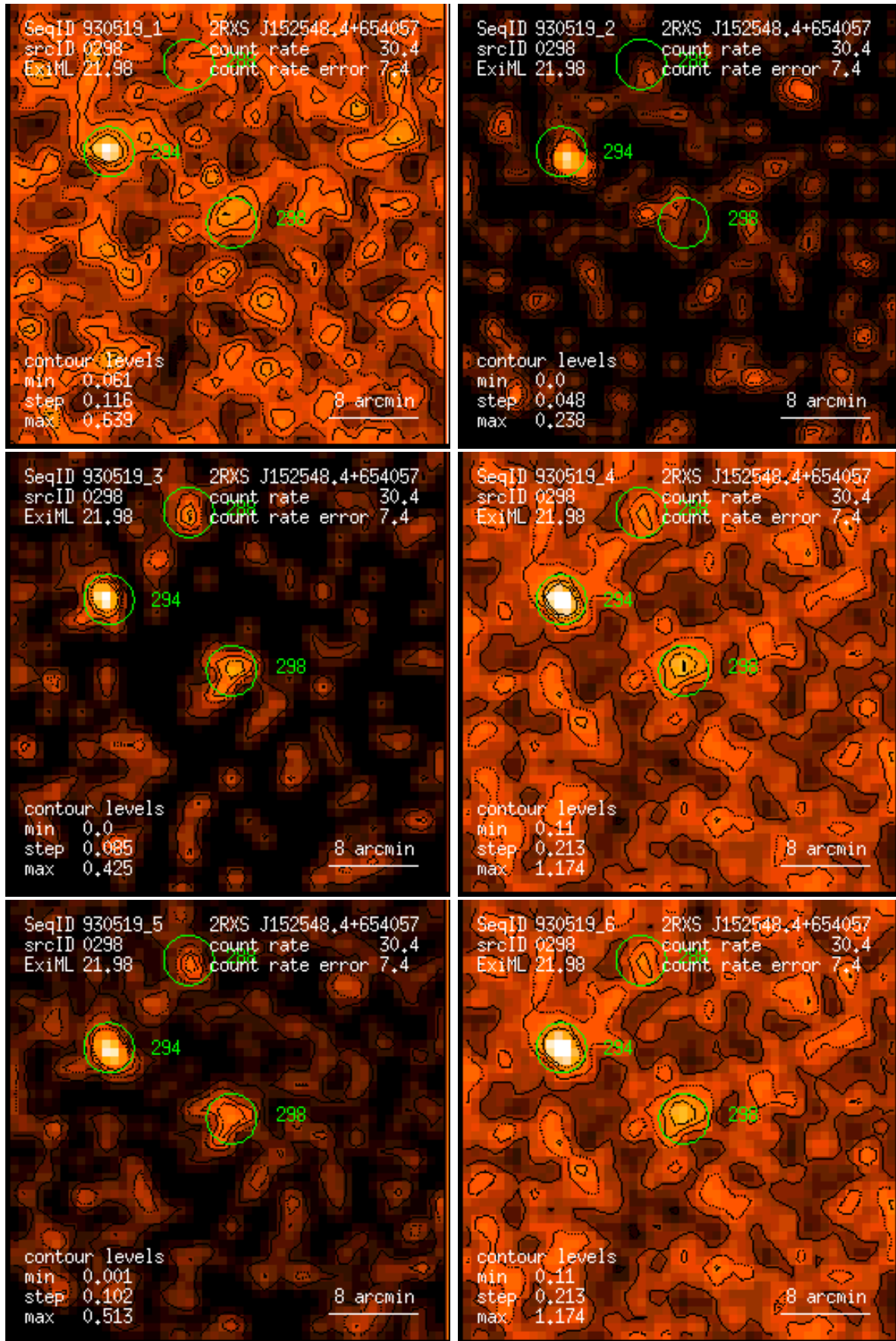
Figure 298: RASS 930519: detection 0298: band rate images, Gaussian filter: (1) PSPC channels 11 – 41, (2) 52 – 90, (3) 91 – 201, (4) 11 – 235, (5) 52 – 201, (6) 11 – 201. Broad band rates in counts/ks. Band rate contour levels in counts/ks/arcmin 2 .
