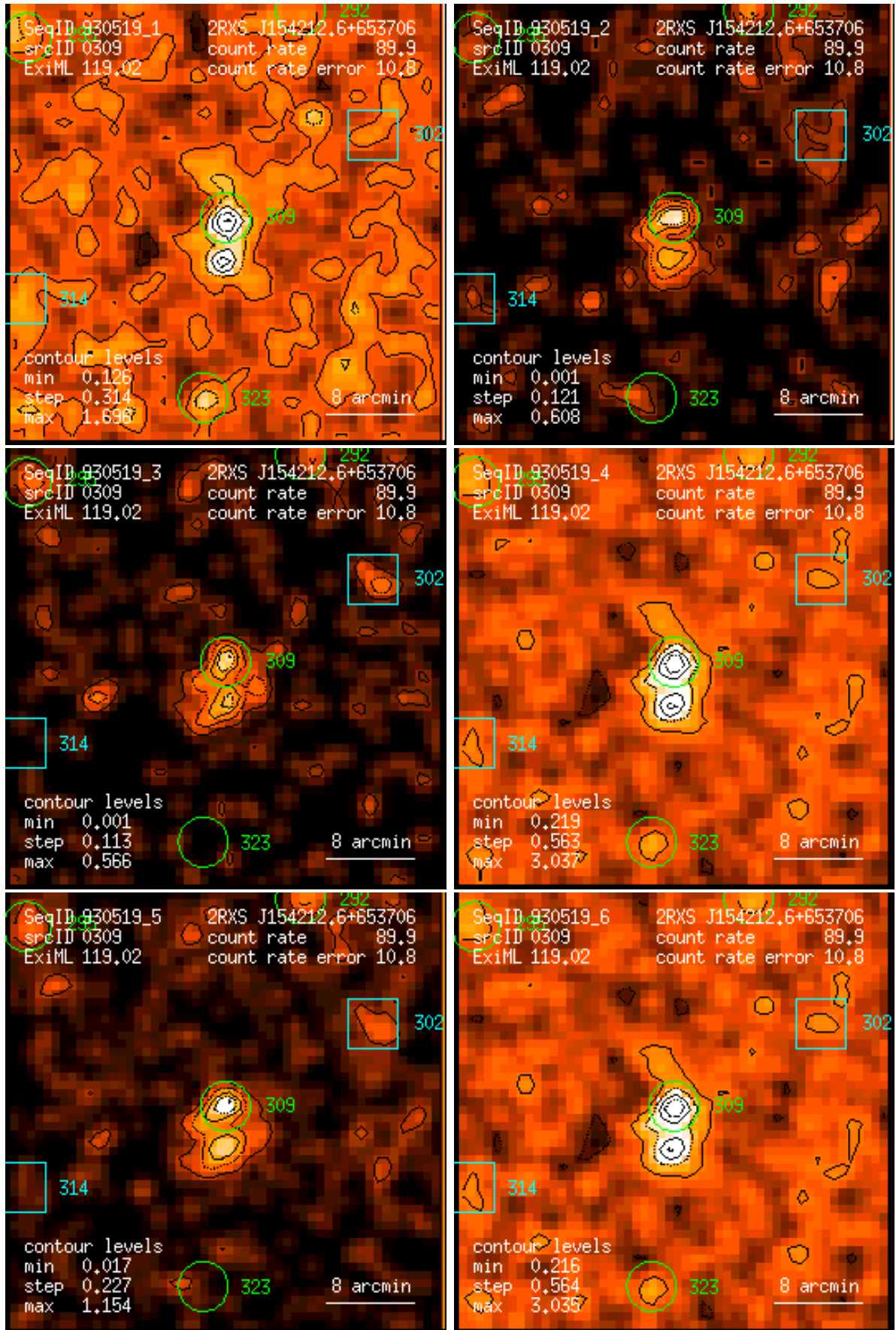
Figure 309: RASS 930519: detection 0309: band rate images, Gaussian filter: (1) PSPC channels 11 – 41, (2) 52 – 90, (3) 91 – 201, (4) 11 – 235, (5) 52 – 201, (6) 11 – 201. Broad band rates in counts/ks. Band rate contour levels in counts/ks/arcmin 2 .
