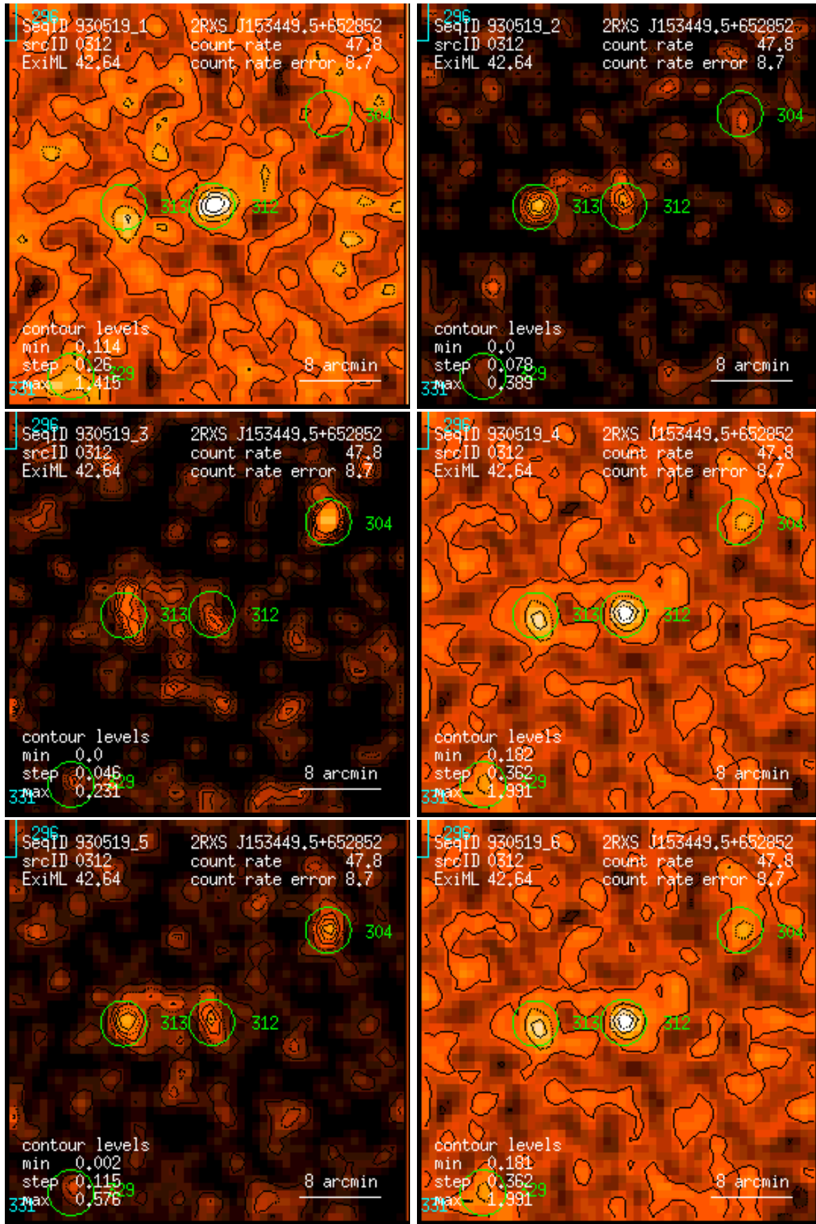
Figure 312: RASS 930519: detection 0312: band rate images, Gaussian filter: (1) PSPC channels 11 – 41, (2) 52 – 90, (3) 91 – 201, (4) 11 – 235, (5) 52 – 201, (6) 11 – 201. Broad band rates in counts/ks. Band rate contour levels in counts/ks/arcmin 2 .
