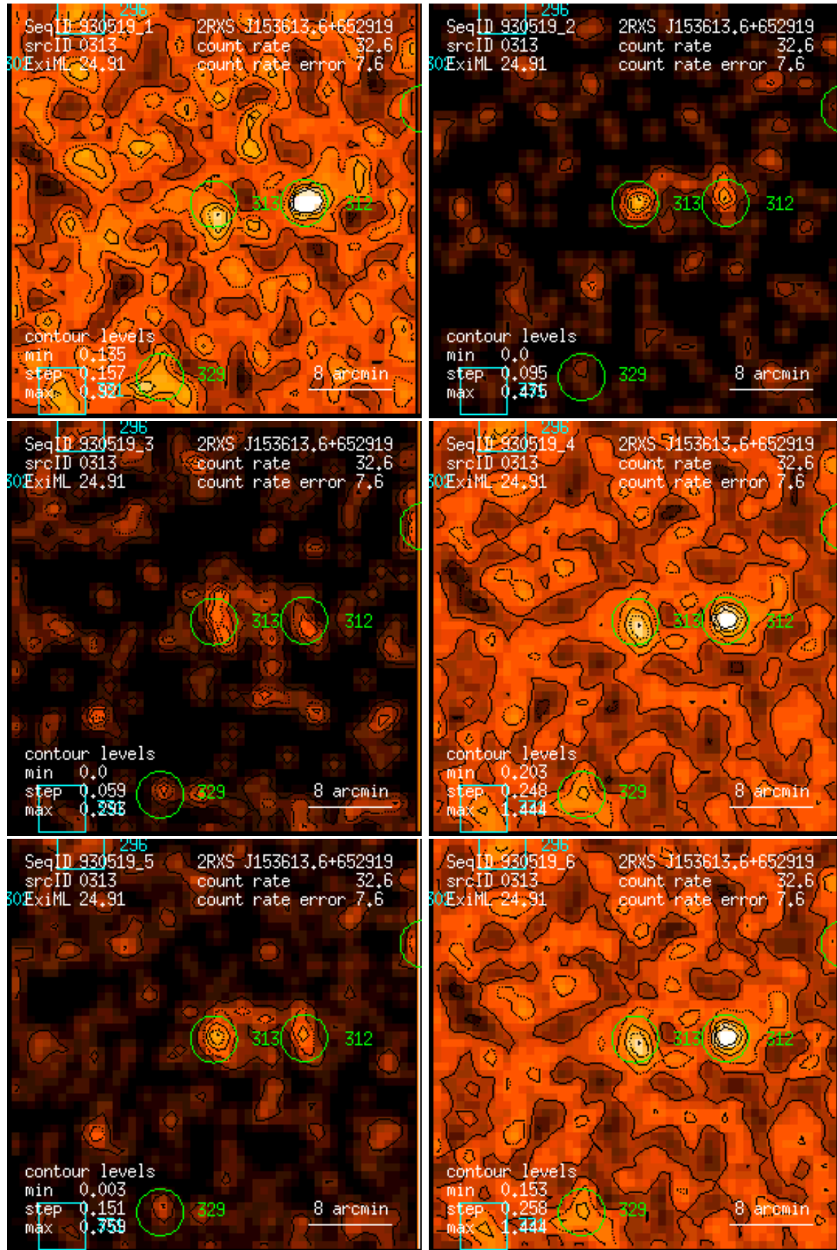
Figure 313: RASS 930519: detection 0313: band rate images, Gaussian filter: (1) PSPC channels 11 – 41, (2) 52 – 90, (3) 91 – 201, (4) 11 – 235, (5) 52 – 201, (6) 11 – 201. Broad band rates in counts/ks. Band rate contour levels in counts/ks/arcmin 2 .
