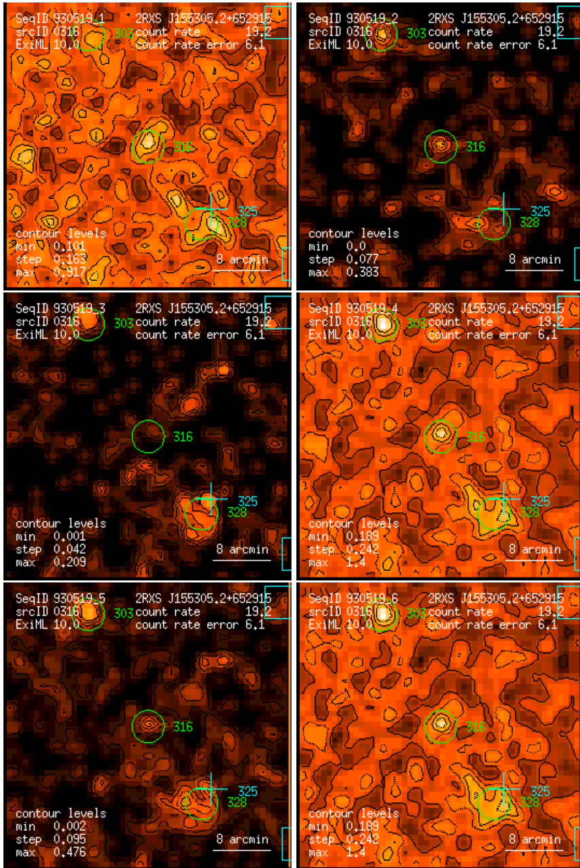
Figure 316: RASS 930519: detection 0316: band rate images, Gaussian filter: (1) PSPC channels 11 – 41, (2) 52 – 90, (3) 91 – 201, (4) 11 – 235, (5) 52 – 201, (6) 11 – 201. Broad band rates in counts/ks. Band rate contour levels in counts/ks/arcmin 2 .
