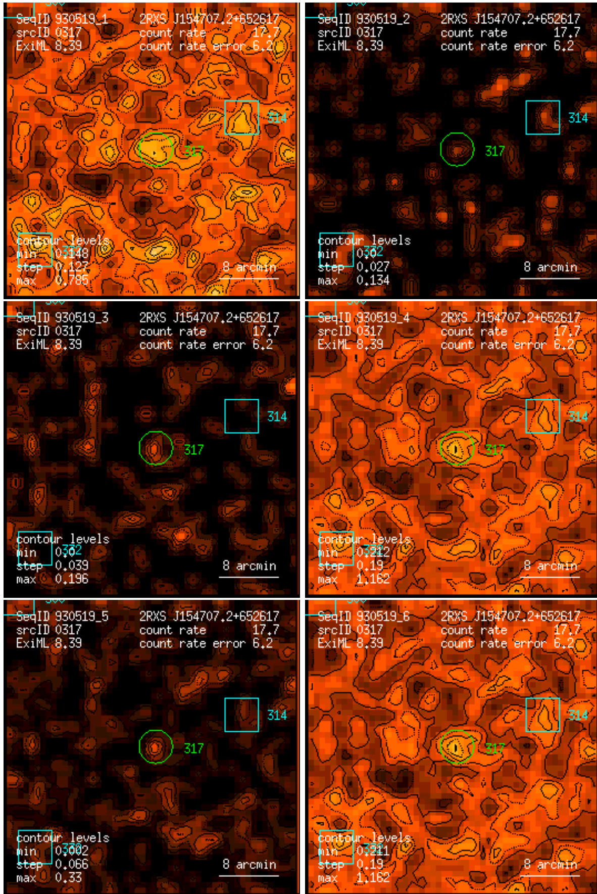
Figure 317: RASS 930519: detection 0317: band rate images, Gaussian filter: (1) PSPC channels 11 – 41, (2) 52 – 90, (3) 91 – 201, (4) 11 – 235, (5) 52 – 201, (6) 11 – 201. Broad band rates in counts/ks. Band rate contour levels in counts/ks/arcmin 2 .
