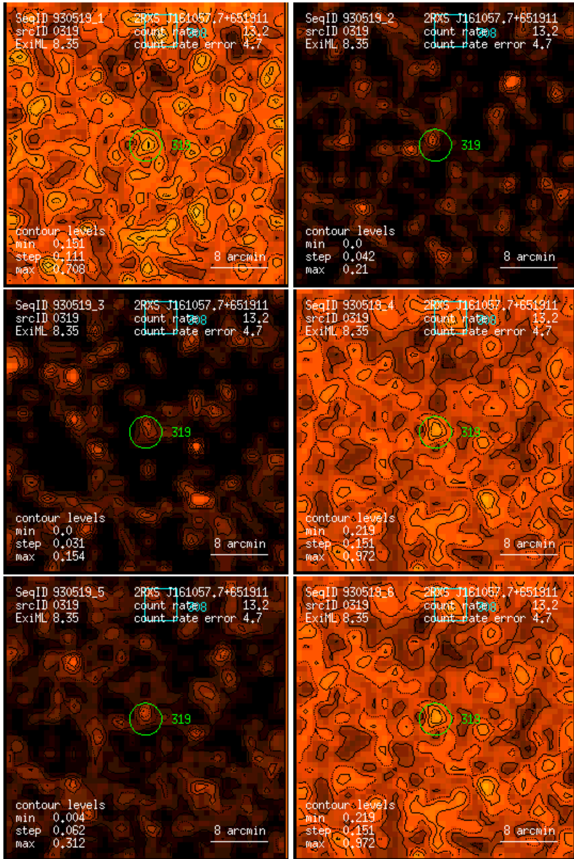
Figure 319: RASS 930519: detection 0319: band rate images, Gaussian filter: (1) PSPC channels 11 – 41, (2) 52 – 90, (3) 91 – 201, (4) 11 – 235, (5) 52 – 201, (6) 11 – 201. Broad band rates in counts/ks. Band rate contour levels in counts/ks/arcmin 2 .
