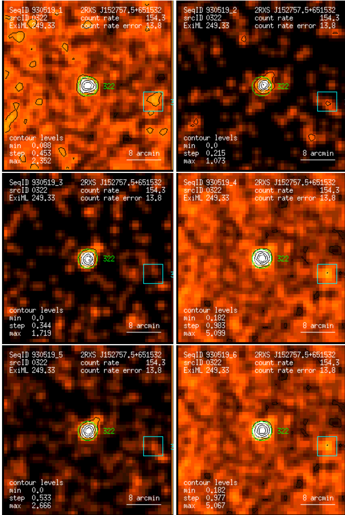
Figure 322: RASS 930519: detection 0322: band rate images, Gaussian filter: (1) PSPC channels 11 – 41, (2) 52 – 90, (3) 91 – 201, (4) 11 – 235, (5) 52 – 201, (6) 11 – 201. Broad band rates in counts/ks. Band rate contour levels in counts/ks/arcmin 2 .
