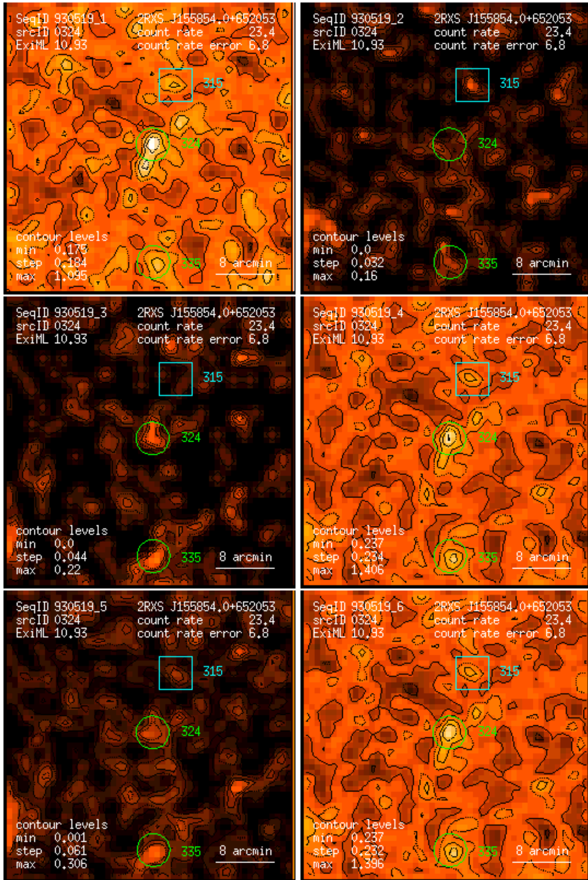
Figure 324: RASS 930519: detection 0324: band rate images, Gaussian filter: (1) PSPC channels 11 – 41, (2) 52 – 90, (3) 91 – 201, (4) 11 – 235, (5) 52 – 201, (6) 11 – 201. Broad band rates in counts/ks. Band rate contour levels in counts/ks/arcmin 2 .
