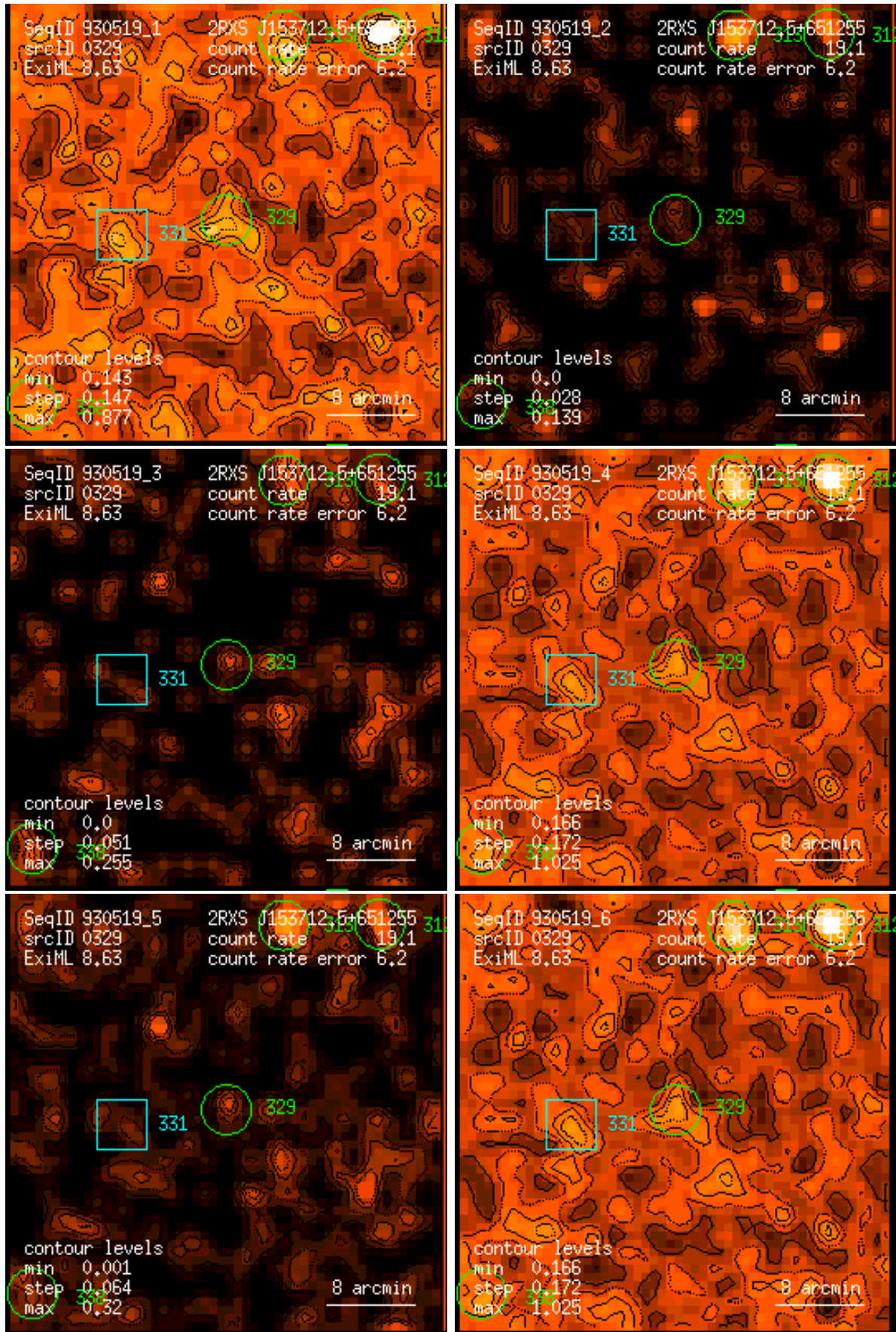
Figure 329: RASS 930519: detection 0329: band rate images, Gaussian filter: (1) PSPC channels 11 – 41, (2) 52 – 90, (3) 91 – 201, (4) 11 – 235, (5) 52 – 201, (6) 11 – 201. Broad band rates in counts/ks. Band rate contour levels in counts/ks/arcmin 2 .
