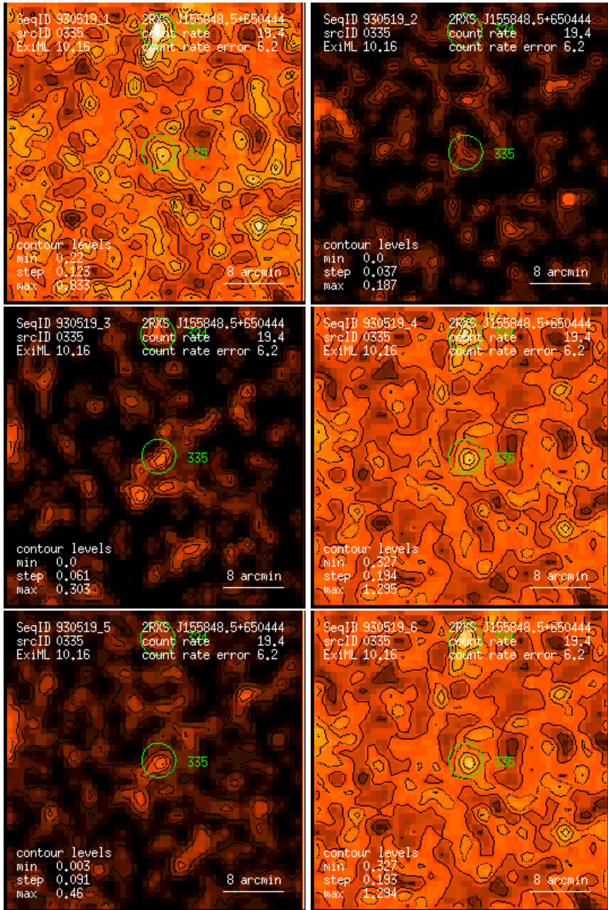
Figure 335: RASS 930519: detection 0335: band rate images, Gaussian filter: (1) PSPC channels 11 – 41, (2) 52 – 90, (3) 91 – 201, (4) 11 – 235, (5) 52 – 201, (6) 11 – 201. Broad band rates in counts/ks. Band rate contour levels in counts/ks/arcmin 2 .
