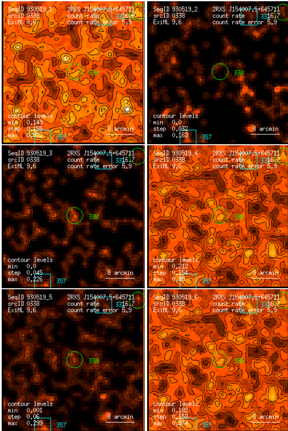
Figure 338: RASS 930519: detection 0338: band rate images, Gaussian filter: (1) PSPC channels 11 – 41, (2) 52 – 90, (3) 91 – 201, (4) 11 – 235, (5) 52 – 201, (6) 11 – 201. Broad band rates in counts/ks. Band rate contour levels in counts/ks/arcmin 2 .
