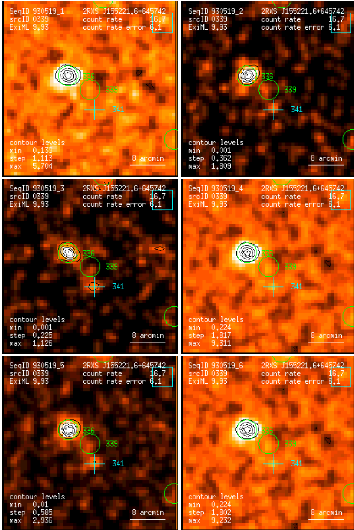
Figure 339: RASS 930519: detection 0339: band rate images, Gaussian filter: (1) PSPC channels 11 – 41, (2) 52 – 90, (3) 91 – 201, (4) 11 – 235, (5) 52 – 201, (6) 11 – 201. Broad band rates in counts/ks. Band rate contour levels in counts/ks/arcmin 2 .
