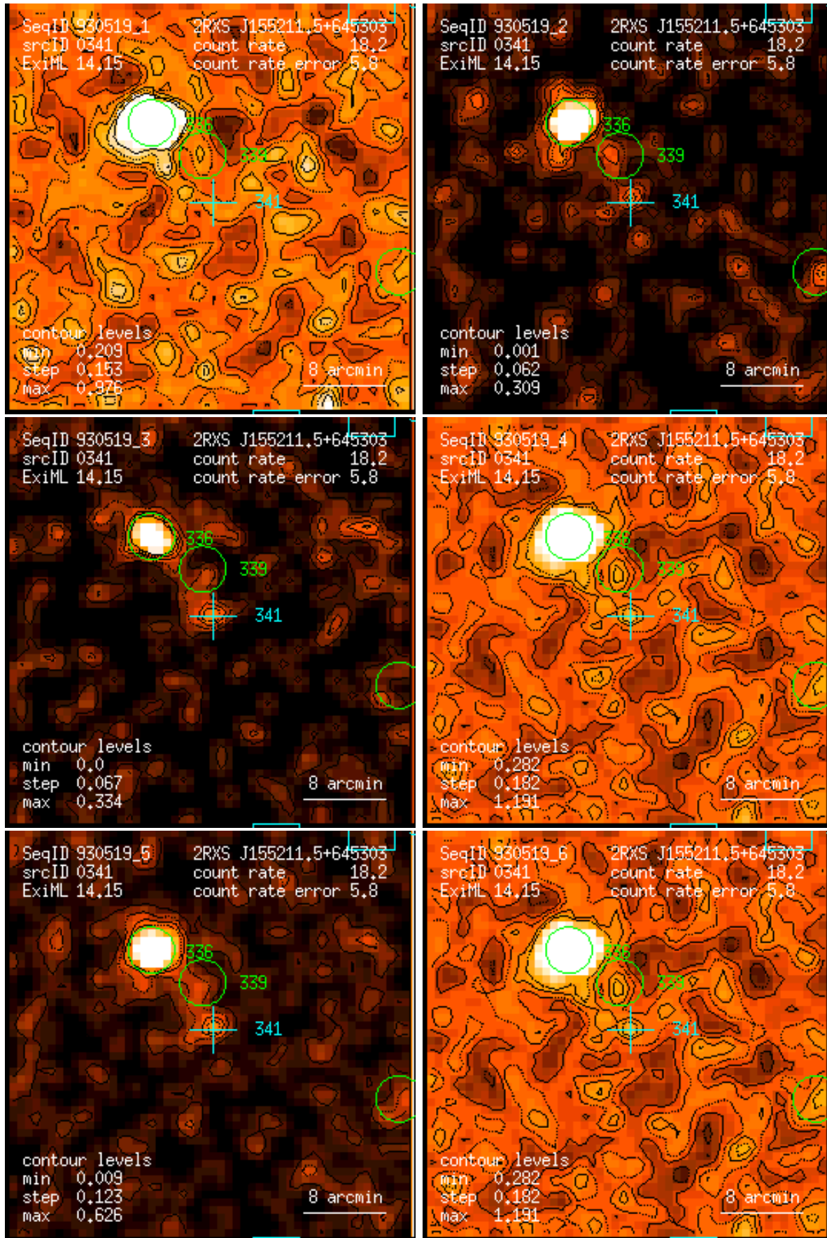
Figure 341: RASS 930519: detection 0341: band rate images, Gaussian filter: (1) PSPC channels 11 – 41, (2) 52 – 90, (3) 91 – 201, (4) 11 – 235, (5) 52 – 201, (6) 11 – 201. Broad band rates in counts/ks. Band rate contour levels in counts/ks/arcmin 2 .
