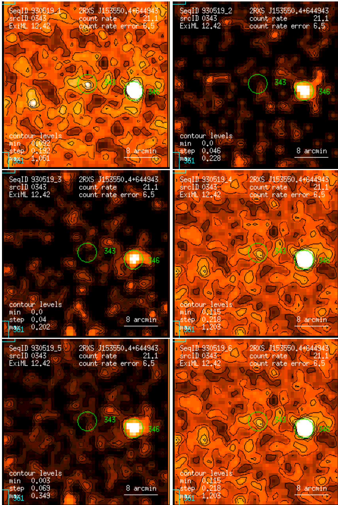
Figure 343: RASS 930519: detection 0343: band rate images, Gaussian filter: (1) PSPC channels 11 – 41, (2) 52 – 90, (3) 91 – 201, (4) 11 – 235, (5) 52 – 201, (6) 11 – 201. Broad band rates in counts/ks. Band rate contour levels in counts/ks/arcmin 2 .
