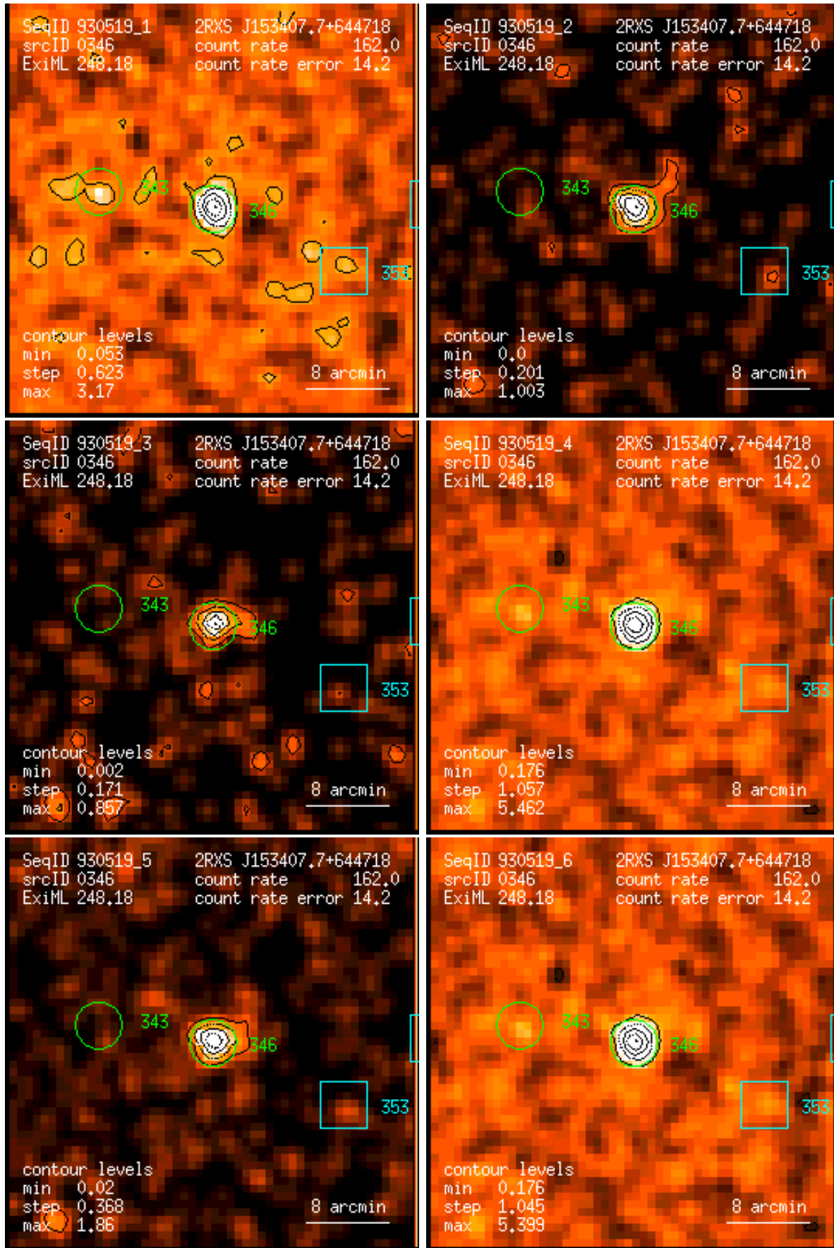
Figure 346: RASS 930519: detection 0346: band rate images, Gaussian filter: (1) PSPC channels 11 – 41, (2) 52 – 90, (3) 91 – 201, (4) 11 – 235, (5) 52 – 201, (6) 11 – 201. Broad band rates in counts/ks. Band rate contour levels in counts/ks/arcmin 2 .
