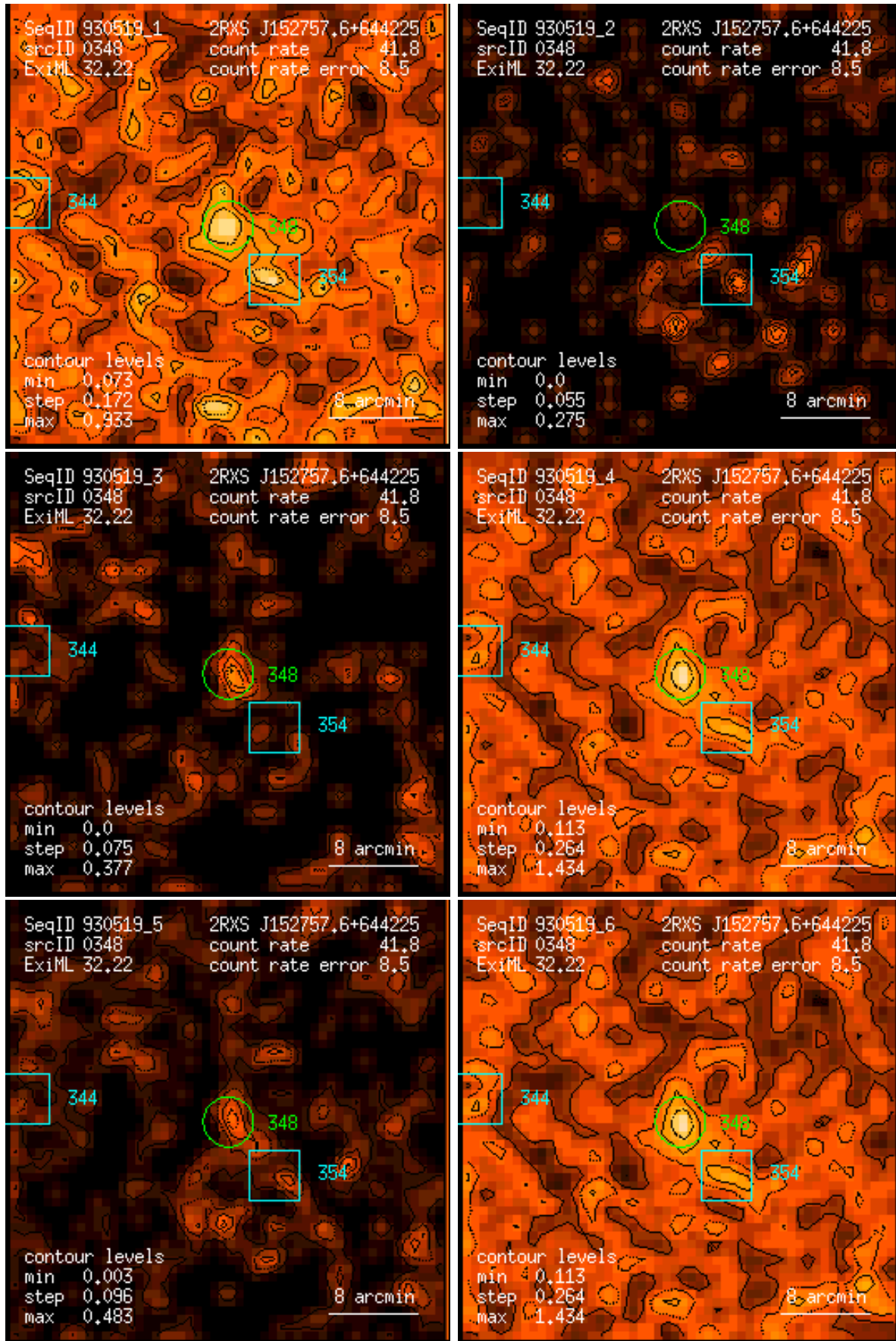
Figure 348: RASS 930519: detection 0348: band rate images, Gaussian filter: (1) PSPC channels 11 – 41, (2) 52 – 90, (3) 91 – 201, (4) 11 – 235, (5) 52 – 201, (6) 11 – 201. Broad band rates in counts/ks. Band rate contour levels in counts/ks/arcmin 2 .
