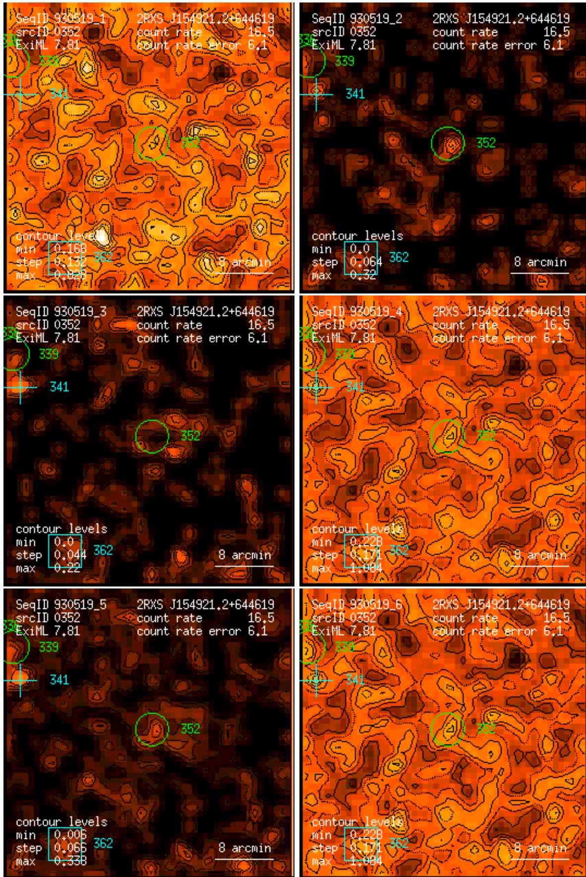
Figure 352: RASS 930519: detection 0352: band rate images, Gaussian filter: (1) PSPC channels 11 – 41, (2) 52 – 90, (3) 91 – 201, (4) 11 – 235, (5) 52 – 201, (6) 11 – 201. Broad band rates in counts/ks. Band rate contour levels in counts/ks/arcmin 2 .
