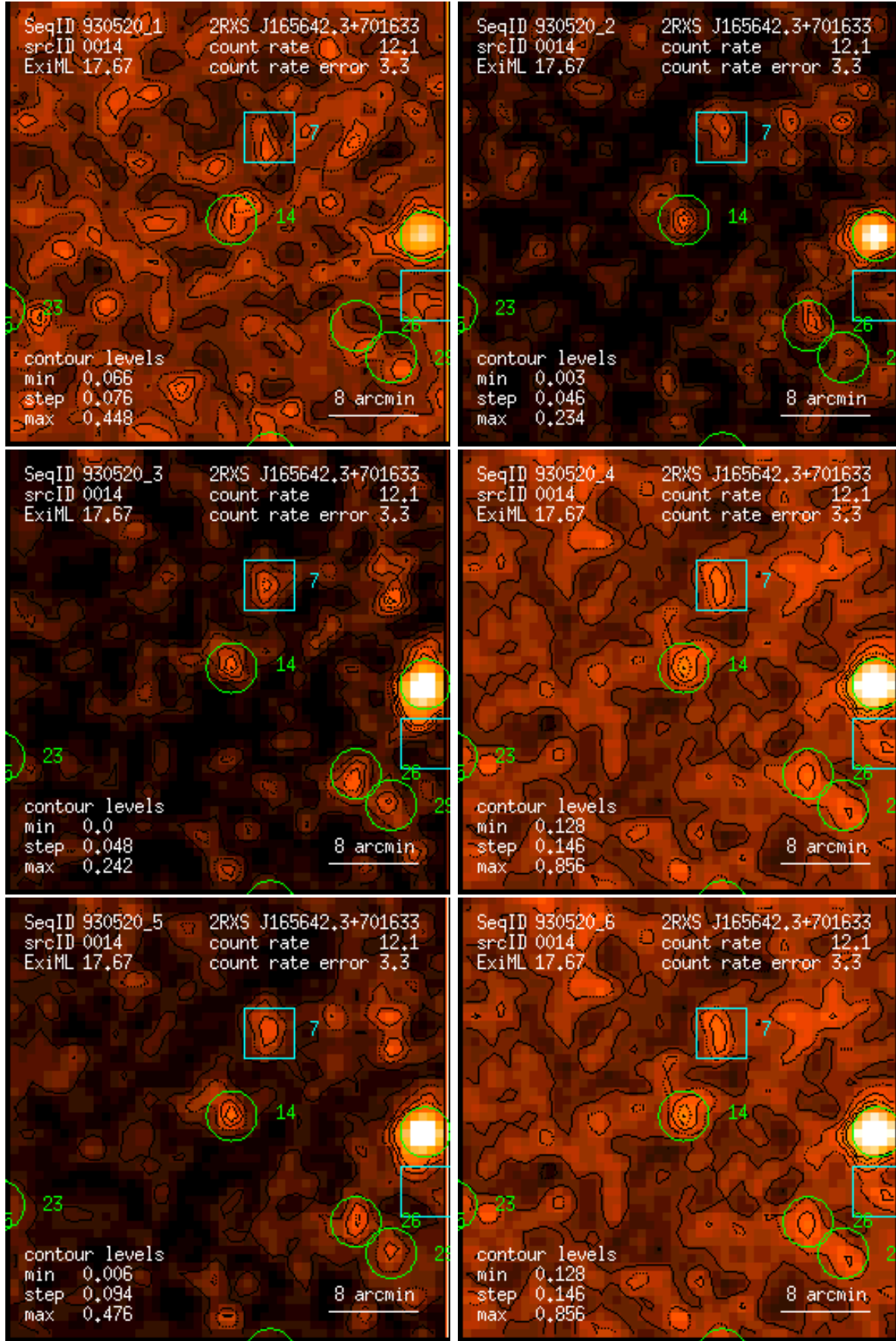
Figure 14: RASS 930520: detection 0014: band rate images, Gaussian filter: (1) PSPC channels 11 – 41, (2) 52 – 90, (3) 91 – 201, (4) 11 – 235, (5) 52 – 201, (6) 11 – 201. Broad band rates in counts/ks. Band rate contour levels in counts/ks/arcmin 2 .
