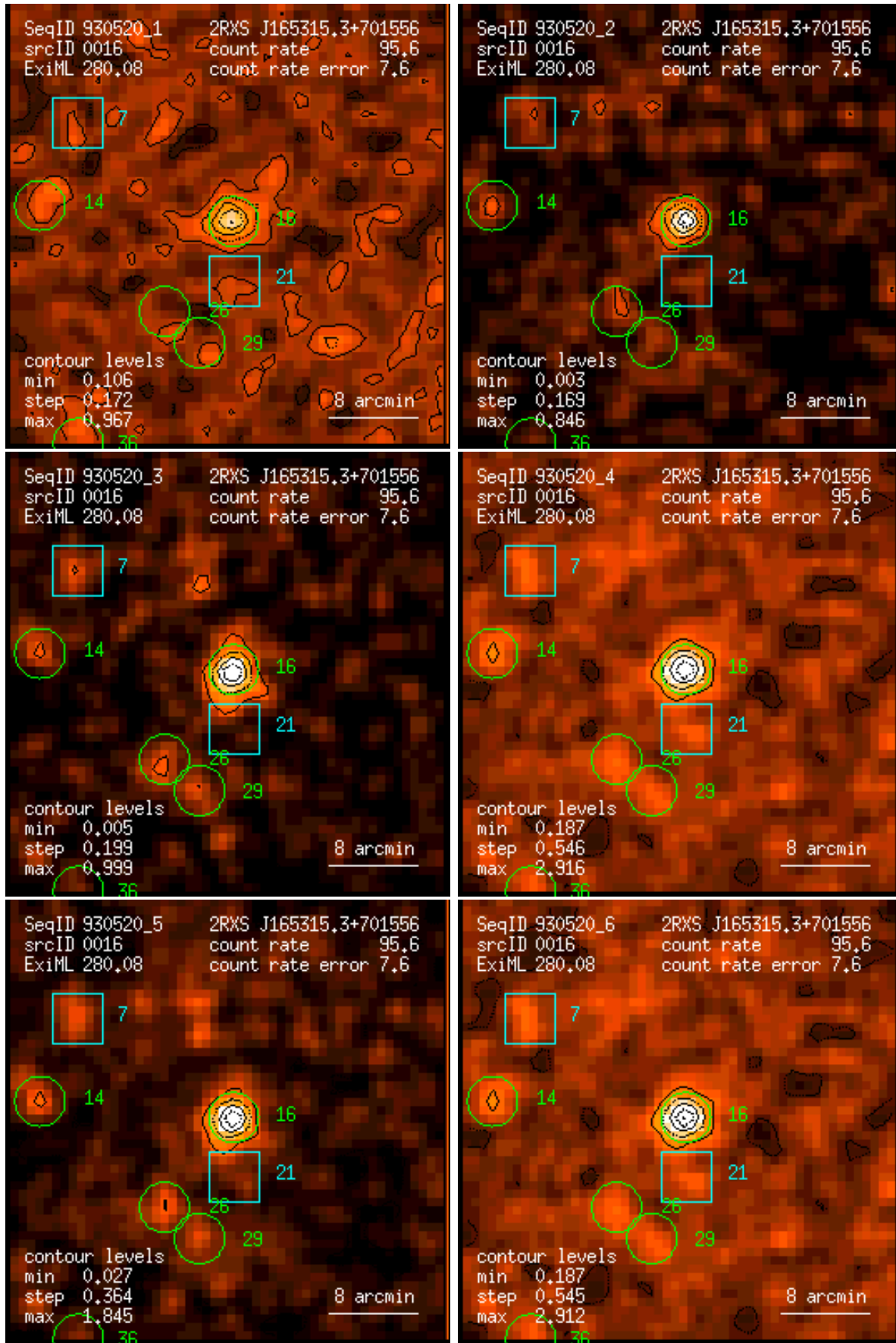
Figure 16: RASS 930520: detection 0016: band rate images, Gaussian filter: (1) PSPC channels 11 – 41, (2) 52 – 90, (3) 91 – 201, (4) 11 – 235, (5) 52 – 201, (6) 11 – 201. Broad band rates in counts/ks. Band rate contour levels in counts/ks/arcmin 2 .
