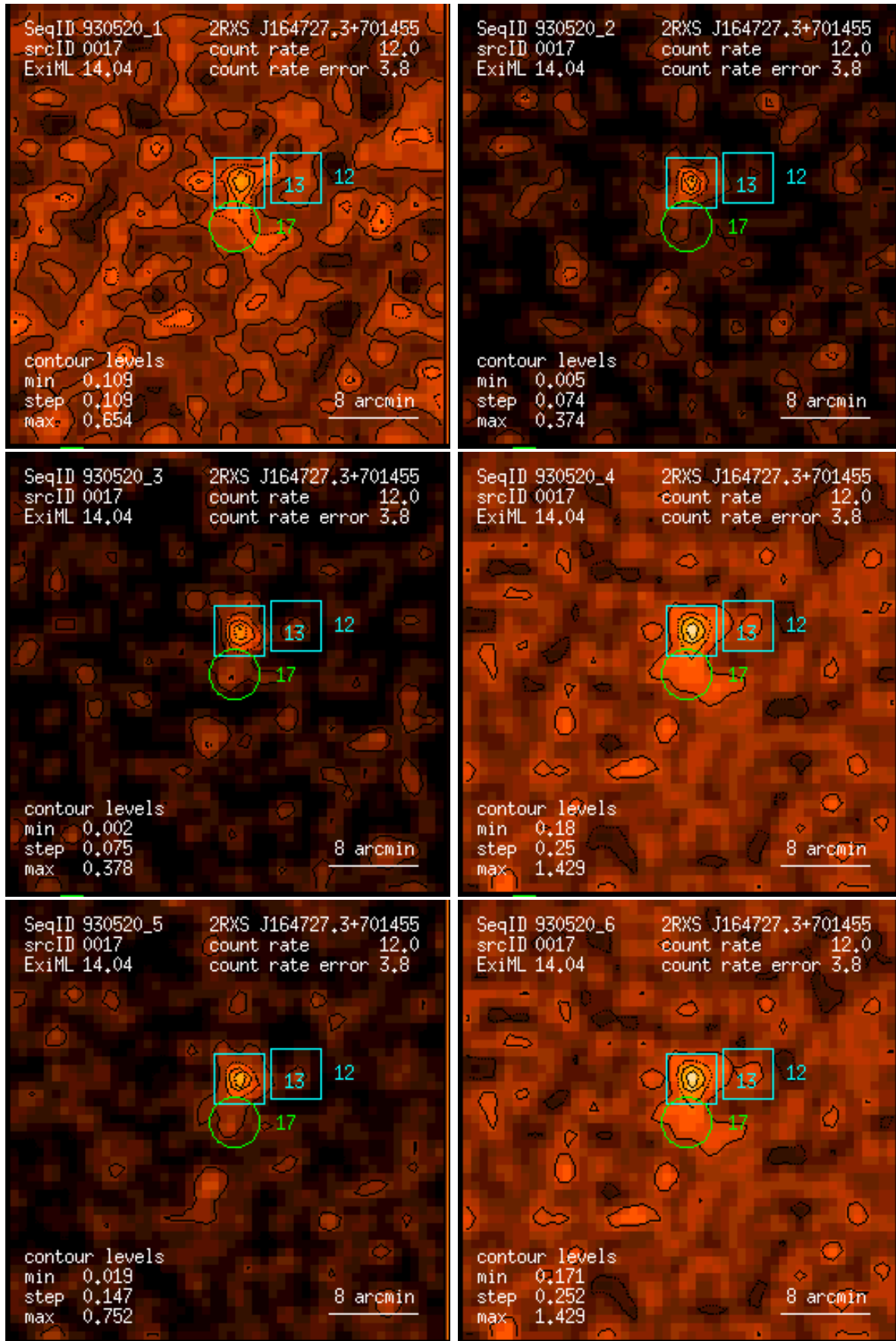
Figure 17: RASS 930520: detection 0017: band rate images, Gaussian filter: (1) PSPC channels 11 – 41, (2) 52 – 90, (3) 91 – 201, (4) 11 – 235, (5) 52 – 201, (6) 11 – 201. Broad band rates in counts/ks. Band rate contour levels in counts/ks/arcmin 2 .
