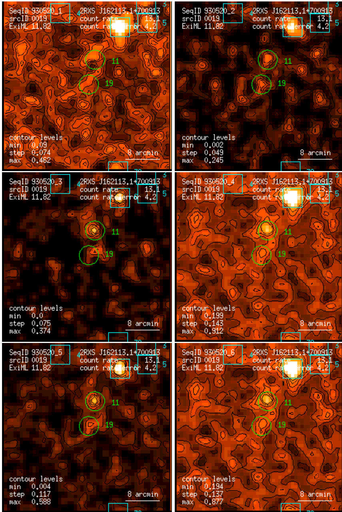
Figure 19: RASS 930520: detection 0019: band rate images, Gaussian filter: (1) PSPC channels 11 – 41, (2) 52 – 90, (3) 91 – 201, (4) 11 – 235, (5) 52 – 201, (6) 11 – 201. Broad band rates in counts/ks. Band rate contour levels in counts/ks/arcmin 2 .
