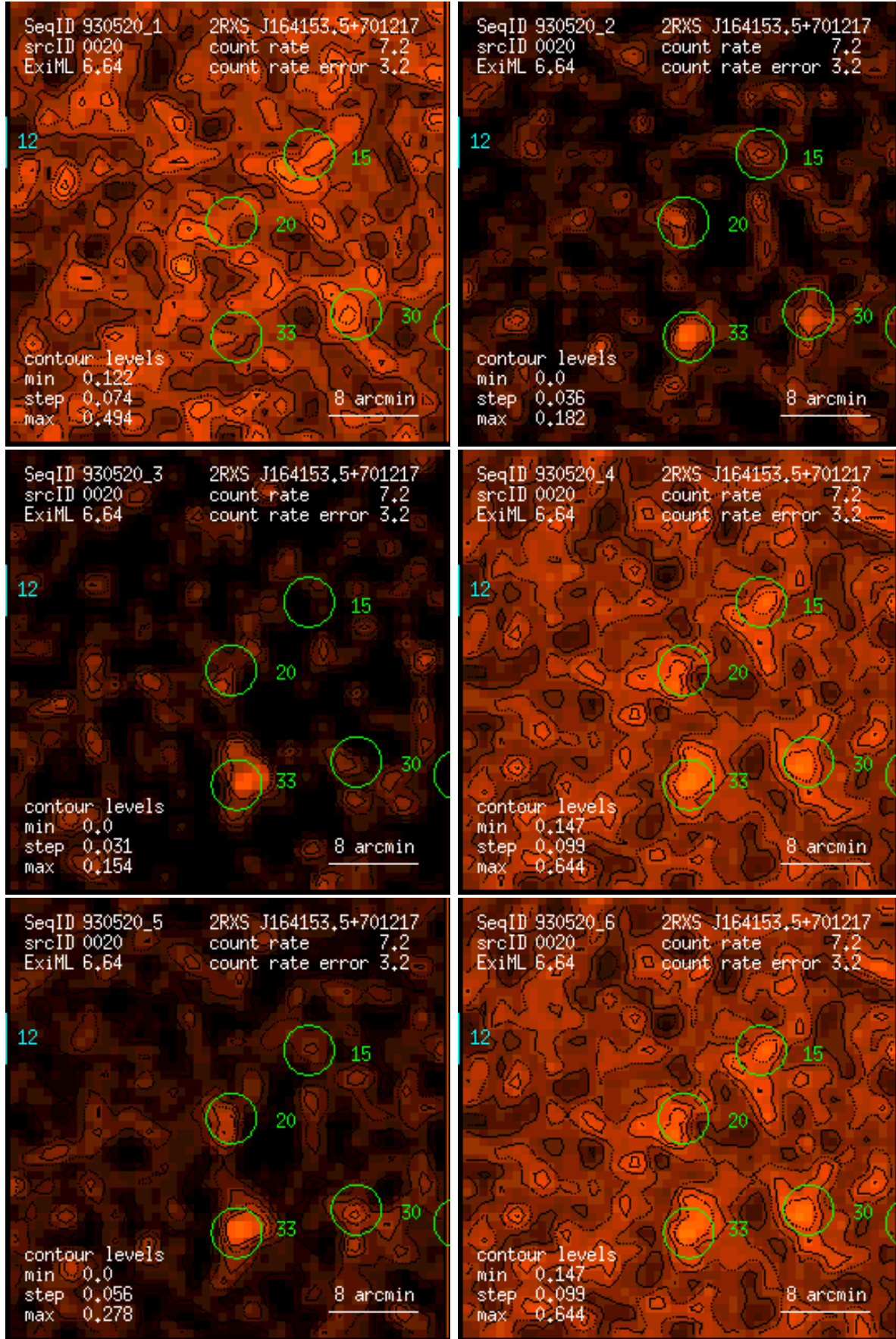
Figure 20: RASS 930520: detection 0020: band rate images, Gaussian filter: (1) PSPC channels 11 – 41, (2) 52 – 90, (3) 91 – 201, (4) 11 – 235, (5) 52 – 201, (6) 11 – 201. Broad band rates in counts/ks. Band rate contour levels in counts/ks/arcmin 2 .
