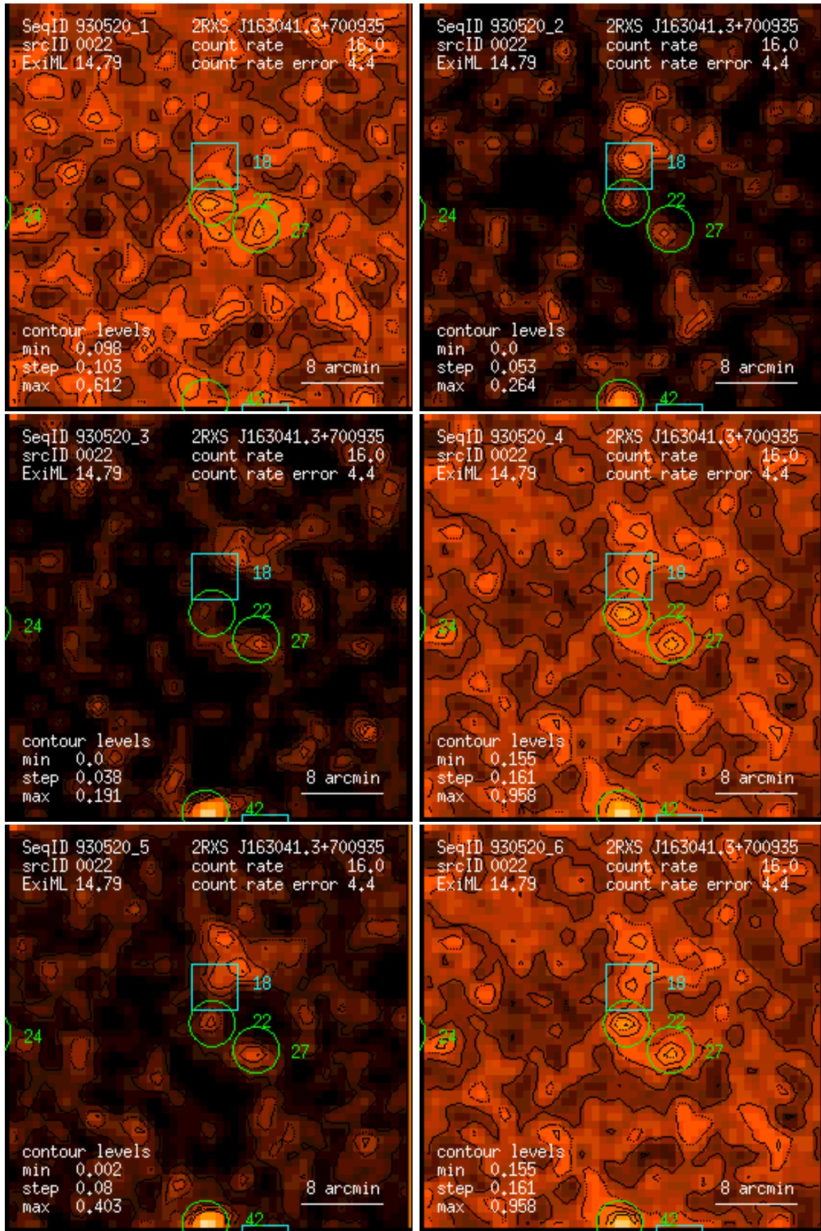
Figure 22: RASS 930520: detection 0022: band rate images, Gaussian filter: (1) PSPC channels 11 – 41, (2) 52 – 90, (3) 91 – 201, (4) 11 – 235, (5) 52 – 201, (6) 11 – 201. Broad band rates in counts/ks. Band rate contour levels in counts/ks/arcmin 2 .
