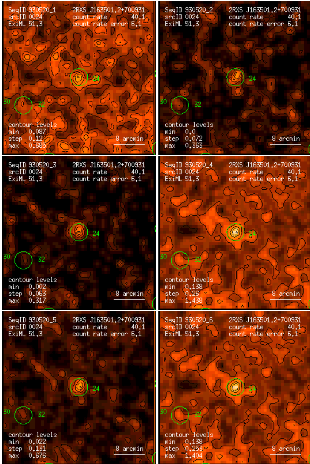
Figure 24: RASS 930520: detection 0024: band rate images, Gaussian filter: (1) PSPC channels 11 – 41, (2) 52 – 90, (3) 91 – 201, (4) 11 – 235, (5) 52 – 201, (6) 11 – 201. Broad band rates in counts/ks. Band rate contour levels in counts/ks/arcmin 2 .
