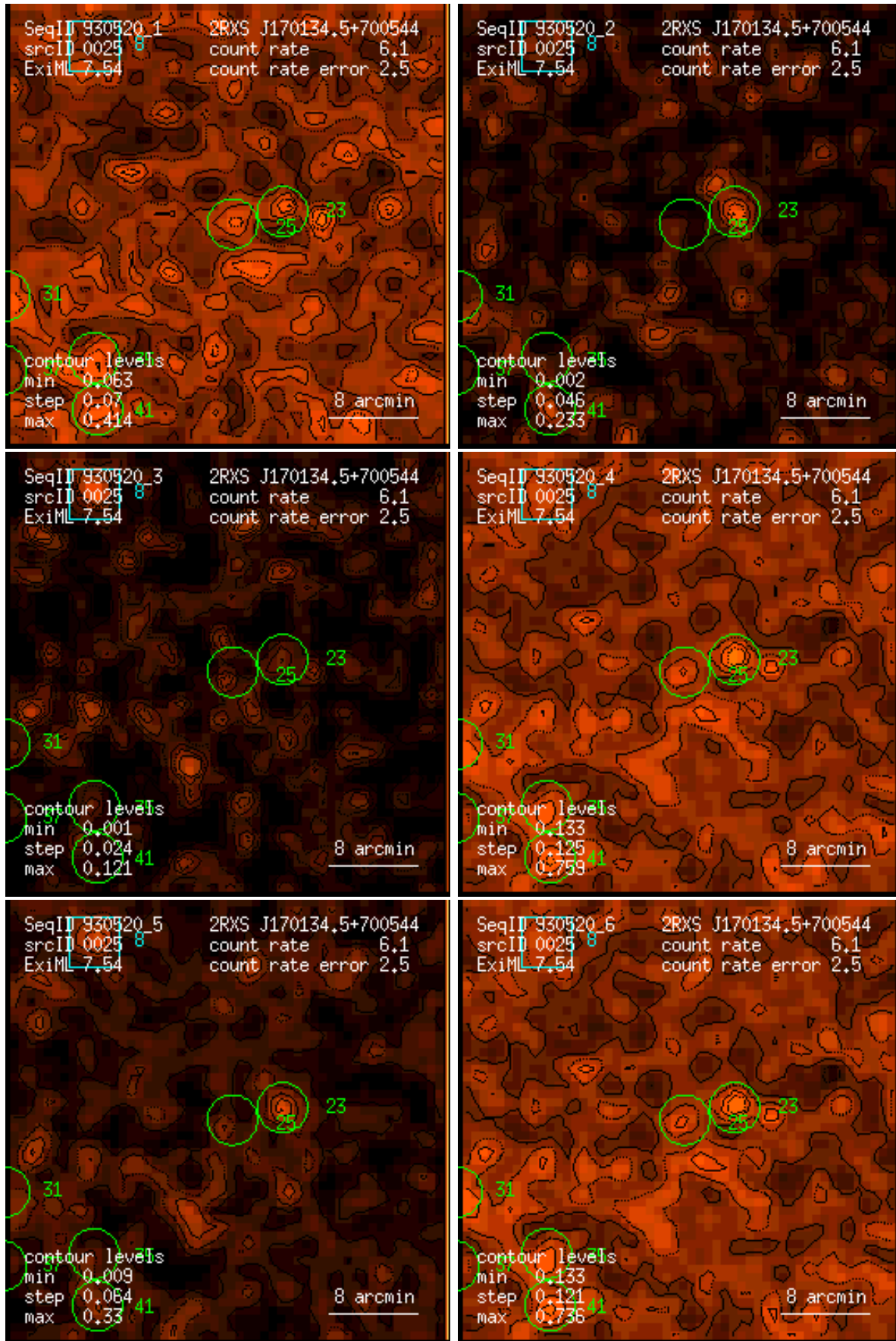
Figure 25: RASS 930520: detection 0025: band rate images, Gaussian filter: (1) PSPC channels 11 – 41, (2) 52 – 90, (3) 91 – 201, (4) 11 – 235, (5) 52 – 201, (6) 11 – 201. Broad band rates in counts/ks. Band rate contour levels in counts/ks/arcmin 2 .
