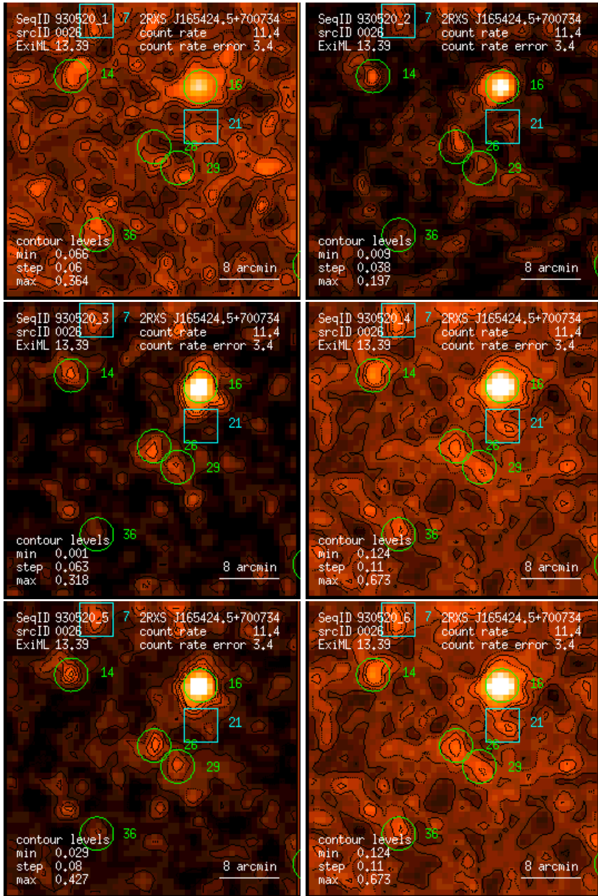
Figure 26: RASS 930520: detection 0026: band rate images, Gaussian filter: (1) PSPC channels 11 – 41, (2) 52 – 90, (3) 91 – 201, (4) 11 – 235, (5) 52 – 201, (6) 11 – 201. Broad band rates in counts/ks. Band rate contour levels in counts/ks/arcmin 2 .
