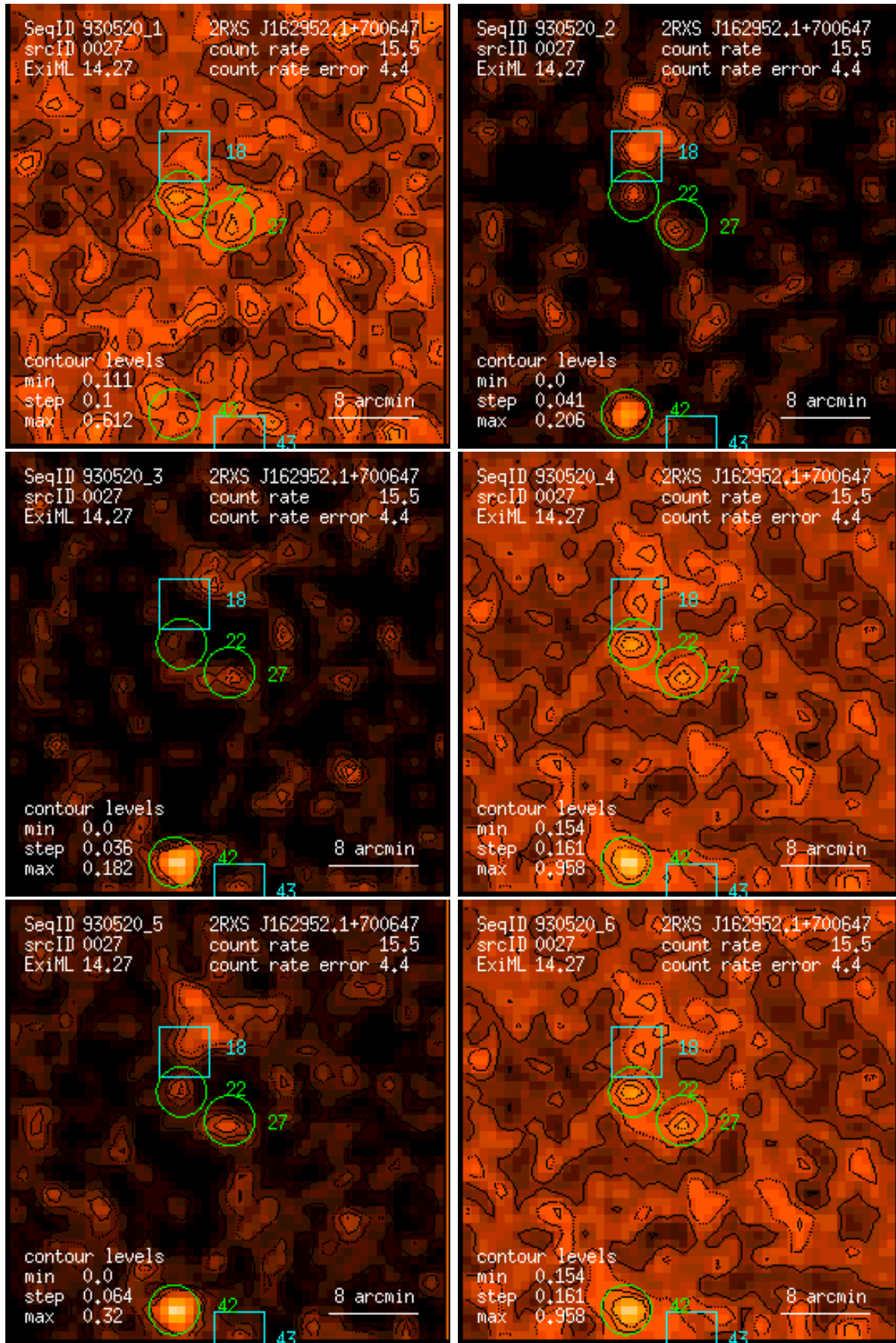
Figure 27: RASS 930520: detection 0027: band rate images, Gaussian filter: (1) PSPC channels 11 – 41, (2) 52 – 90, (3) 91 – 201, (4) 11 – 235, (5) 52 – 201, (6) 11 – 201. Broad band rates in counts/ks. Band rate contour levels in counts/ks/arcmin 2 .
