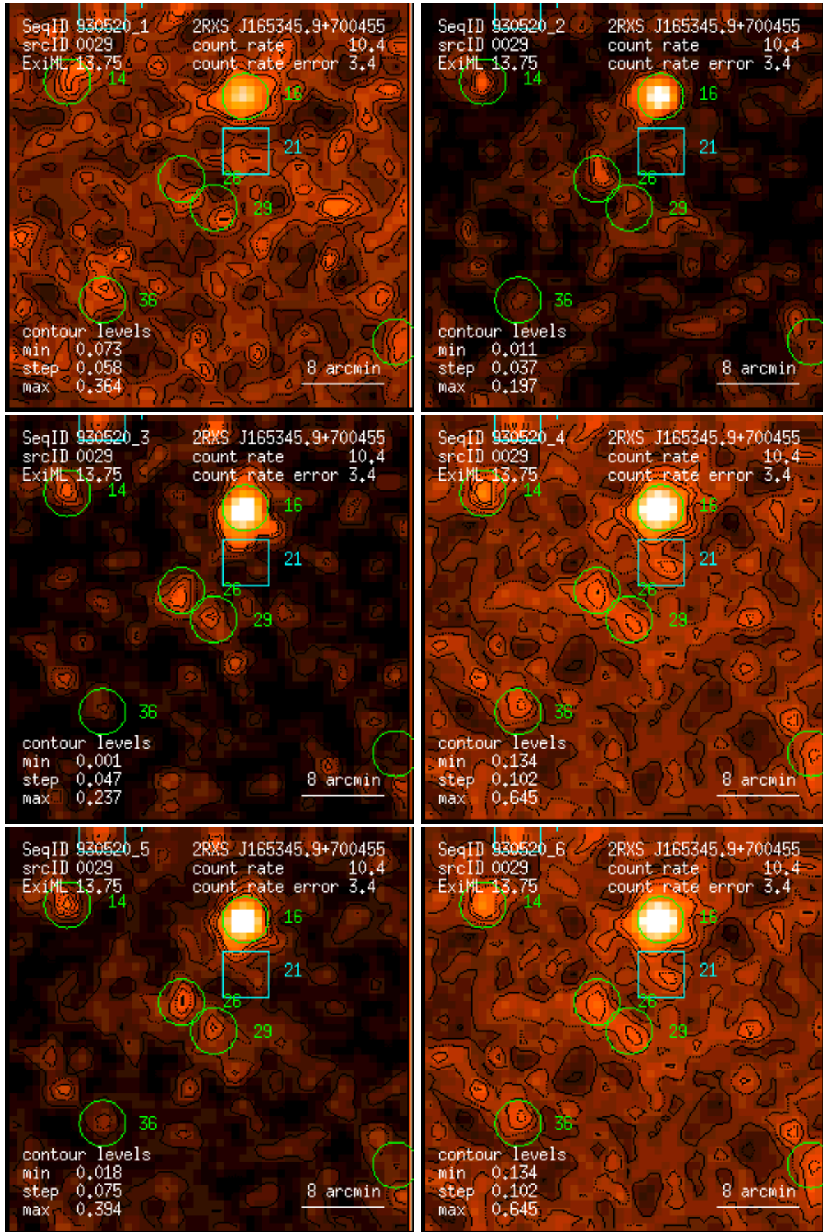
Figure 29: RASS 930520: detection 0029: band rate images, Gaussian filter: (1) PSPC channels 11 – 41, (2) 52 – 90, (3) 91 – 201, (4) 11 – 235, (5) 52 – 201, (6) 11 – 201. Broad band rates in counts/ks. Band rate contour levels in counts/ks/arcmin 2 .
