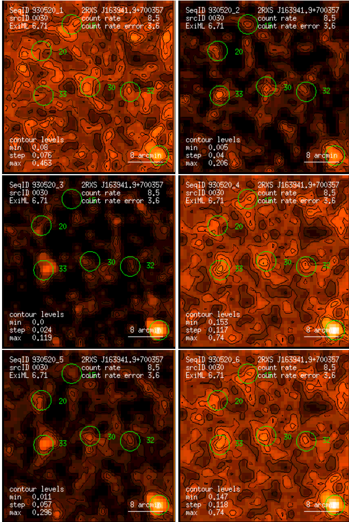
Figure 30: RASS 930520: detection 0030: band rate images, Gaussian filter: (1) PSPC channels 11 – 41, (2) 52 – 90, (3) 91 – 201, (4) 11 – 235, (5) 52 – 201, (6) 11 – 201. Broad band rates in counts/ks. Band rate contour levels in counts/ks/arcmin 2 .
