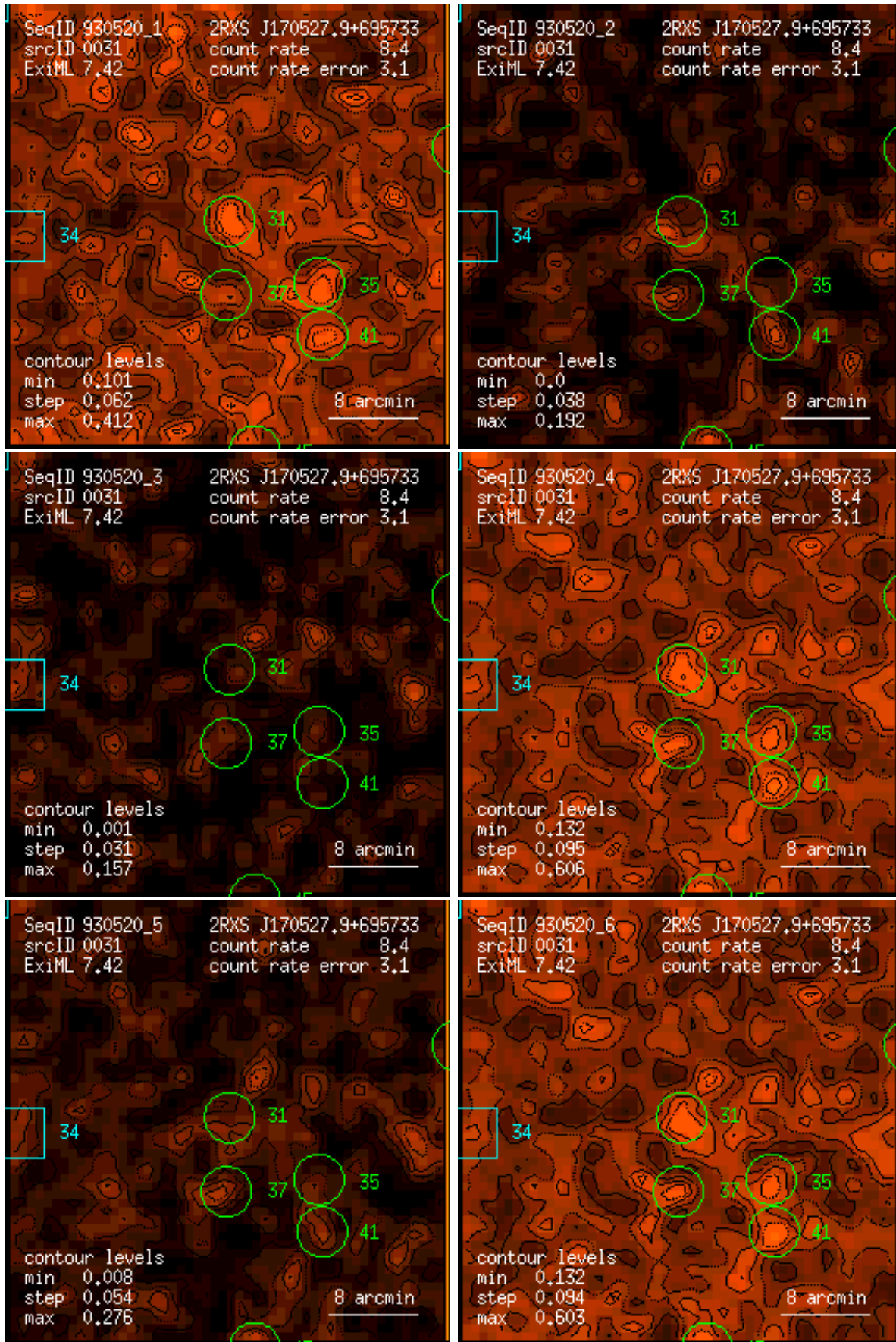
Figure 31: RASS 930520: detection 0031: band rate images, Gaussian filter: (1) PSPC channels 11 – 41, (2) 52 – 90, (3) 91 – 201, (4) 11 – 235, (5) 52 – 201, (6) 11 – 201. Broad band rates in counts/ks. Band rate contour levels in counts/ks/arcmin 2 .
