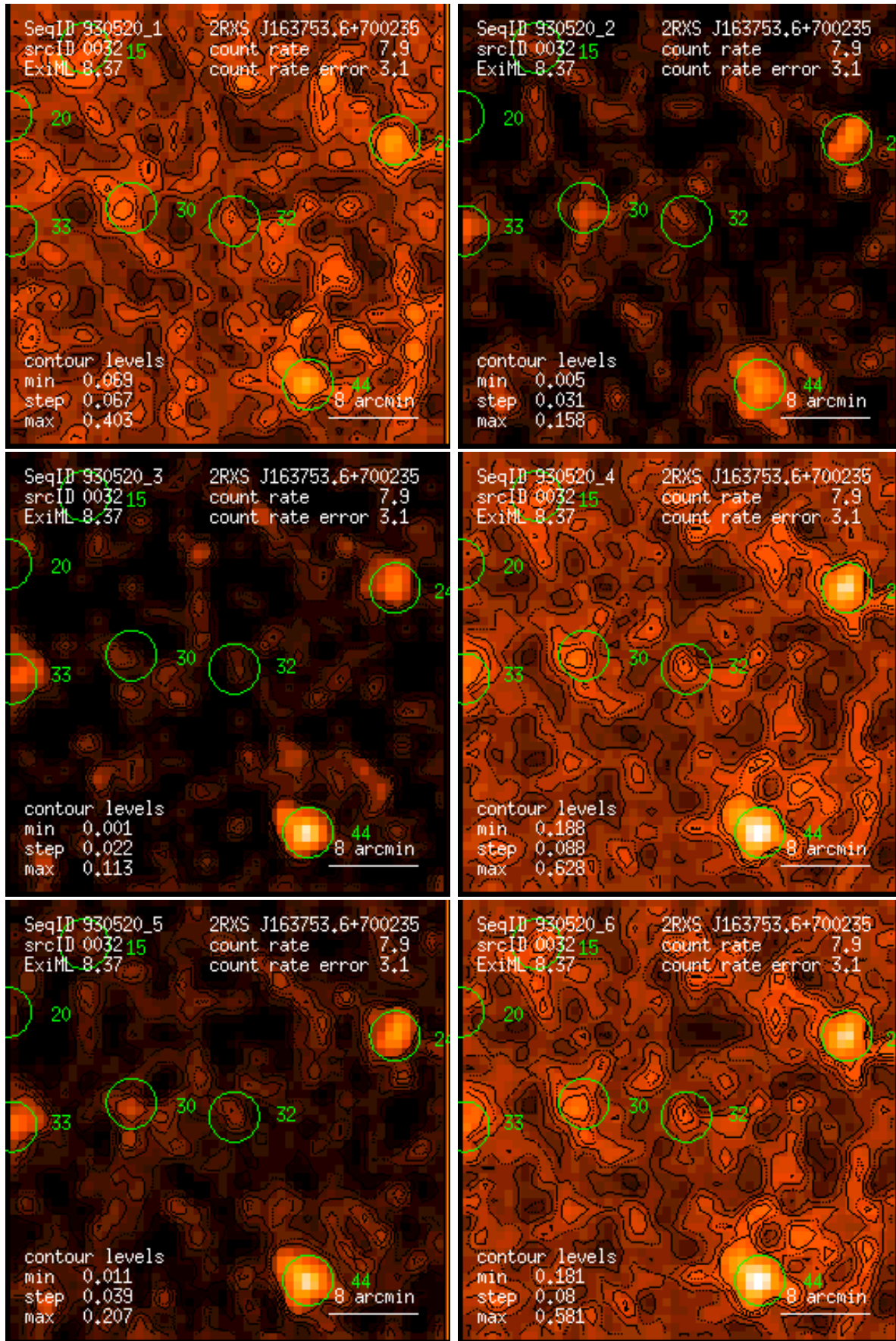
Figure 32: RASS 930520: detection 0032: band rate images, Gaussian filter: (1) PSPC channels 11 – 41, (2) 52 – 90, (3) 91 – 201, (4) 11 – 235, (5) 52 – 201, (6) 11 – 201. Broad band rates in counts/ks. Band rate contour levels in counts/ks/arcmin 2 .
