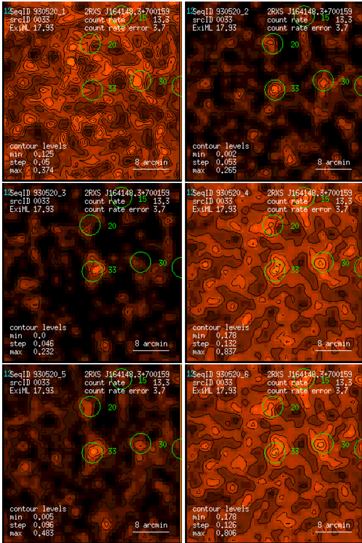
Figure 33: RASS 930520: detection 0033: band rate images, Gaussian filter: (1) PSPC channels 11 – 41, (2) 52 – 90, (3) 91 – 201, (4) 11 – 235, (5) 52 – 201, (6) 11 – 201. Broad band rates in counts/ks. Band rate contour levels in counts/ks/arcmin 2 .
