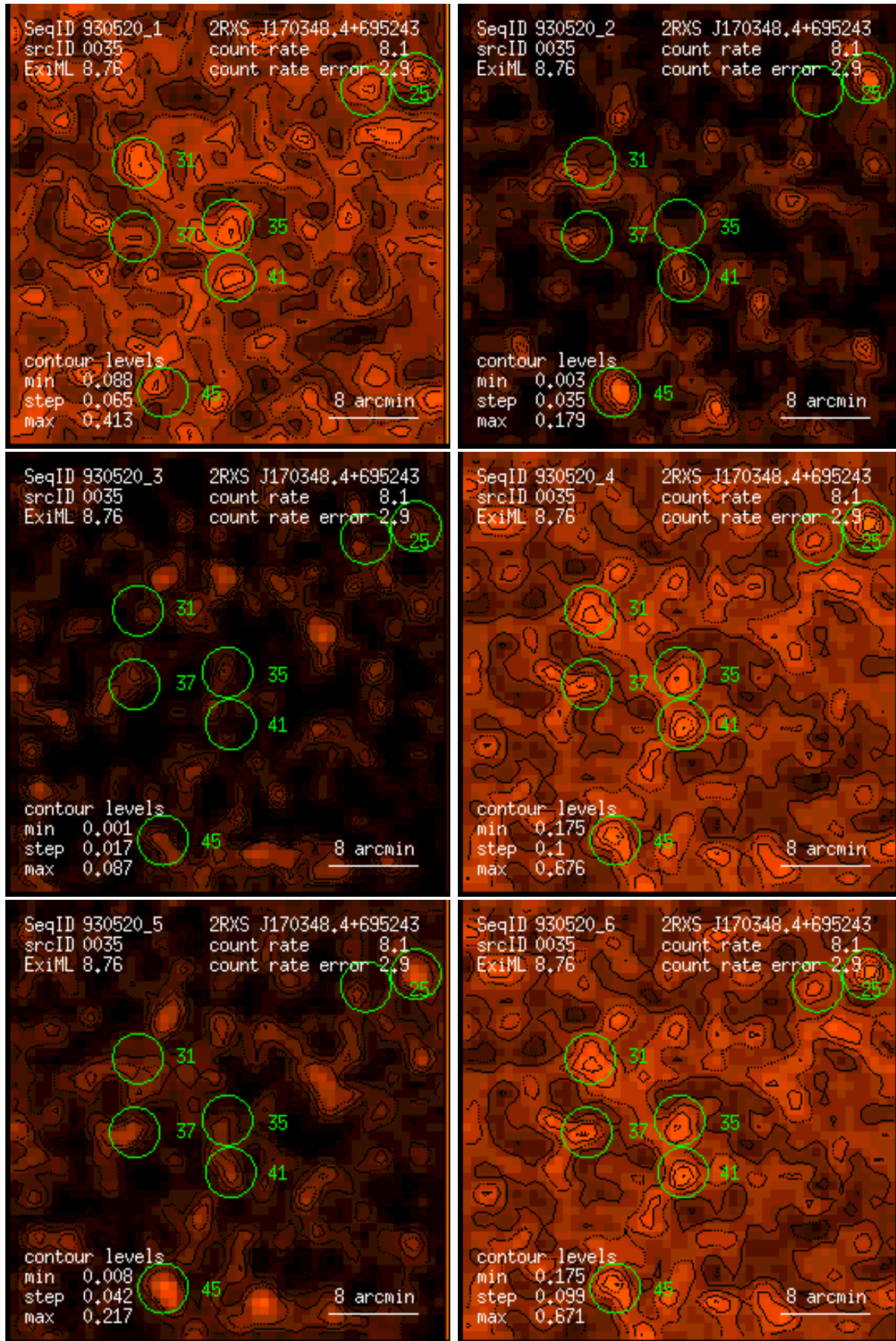
Figure 35: RASS 930520: detection 0035: band rate images, Gaussian filter: (1) PSPC channels 11 – 41, (2) 52 – 90, (3) 91 – 201, (4) 11 – 235, (5) 52 – 201, (6) 11 – 201. Broad band rates in counts/ks. Band rate contour levels in counts/ks/arcmin 2 .
