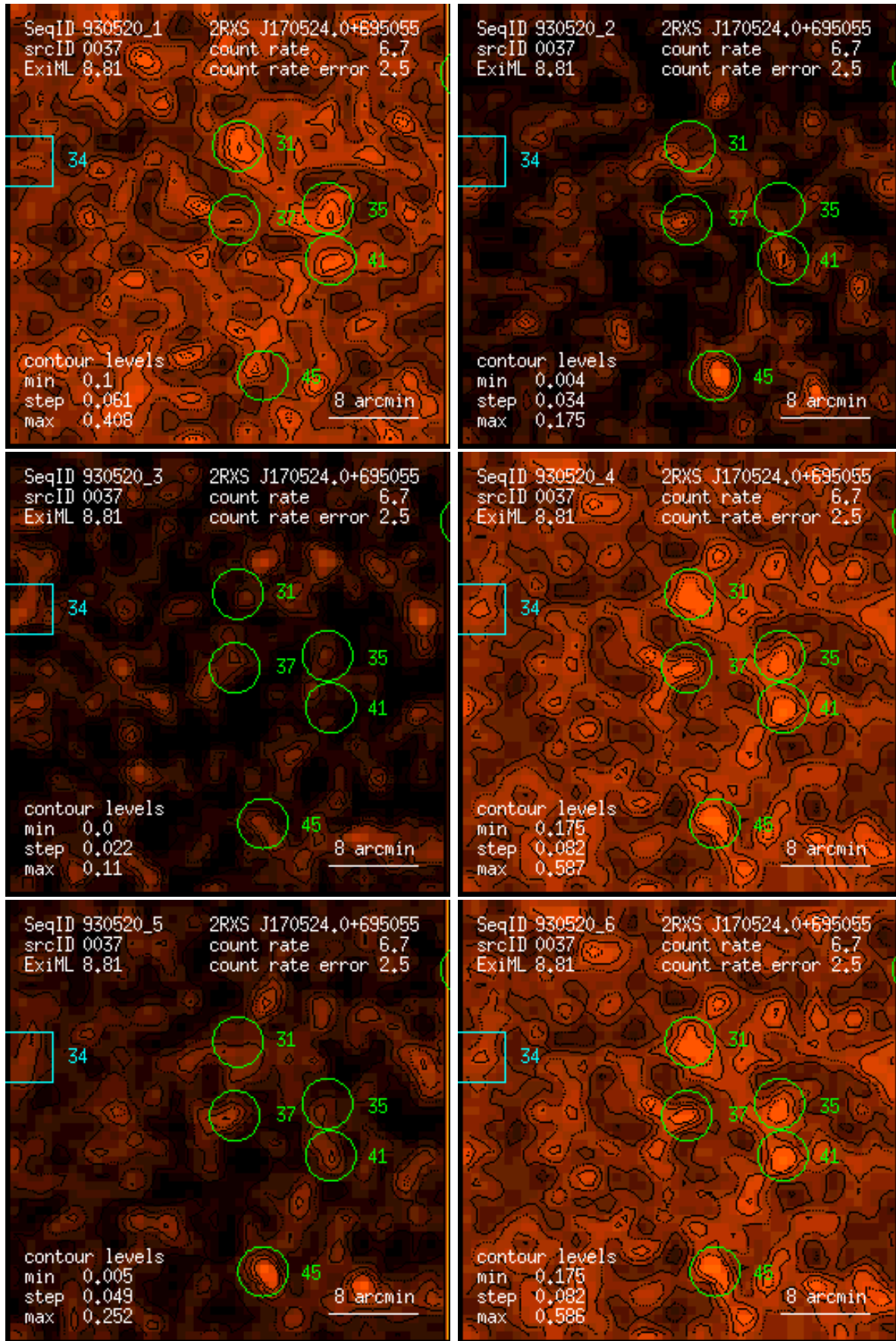
Figure 37: RASS 930520: detection 0037: band rate images, Gaussian filter: (1) PSPC channels 11 – 41, (2) 52 – 90, (3) 91 – 201, (4) 11 – 235, (5) 52 – 201, (6) 11 – 201. Broad band rates in counts/ks. Band rate contour levels in counts/ks/arcmin 2 .
