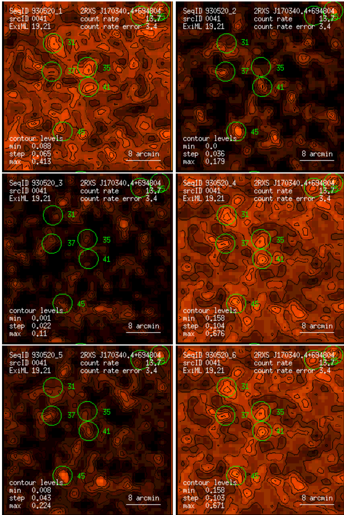
Figure 41: RASS 930520: detection 0041: band rate images, Gaussian filter: (1) PSPC channels 11 – 41, (2) 52 – 90, (3) 91 – 201, (4) 11 – 235, (5) 52 – 201, (6) 11 – 201. Broad band rates in counts/ks. Band rate contour levels in counts/ks/arcmin 2 .
