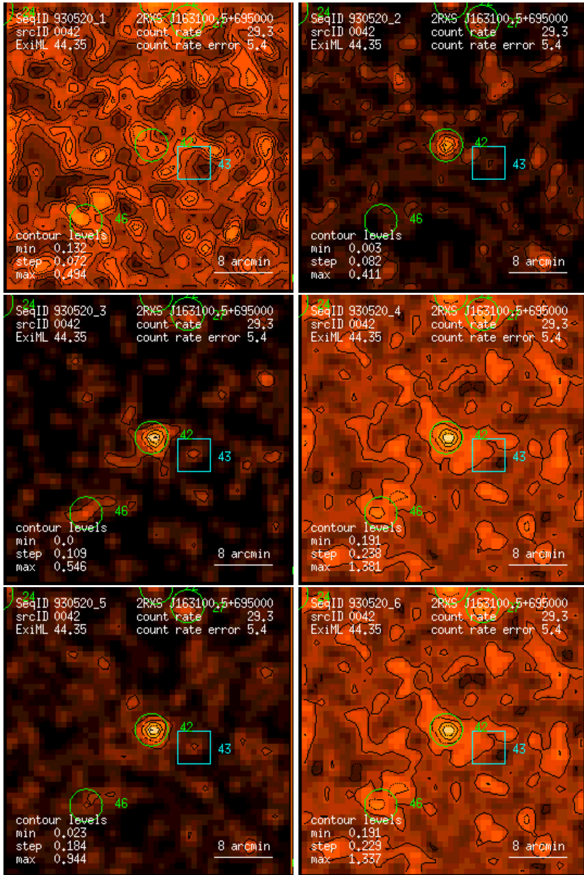
Figure 42: RASS 930520: detection 0042: band rate images, Gaussian filter: (1) PSPC channels 11 – 41, (2) 52 – 90, (3) 91 – 201, (4) 11 – 235, (5) 52 – 201, (6) 11 – 201. Broad band rates in counts/ks. Band rate contour levels in counts/ks/arcmin 2 .
