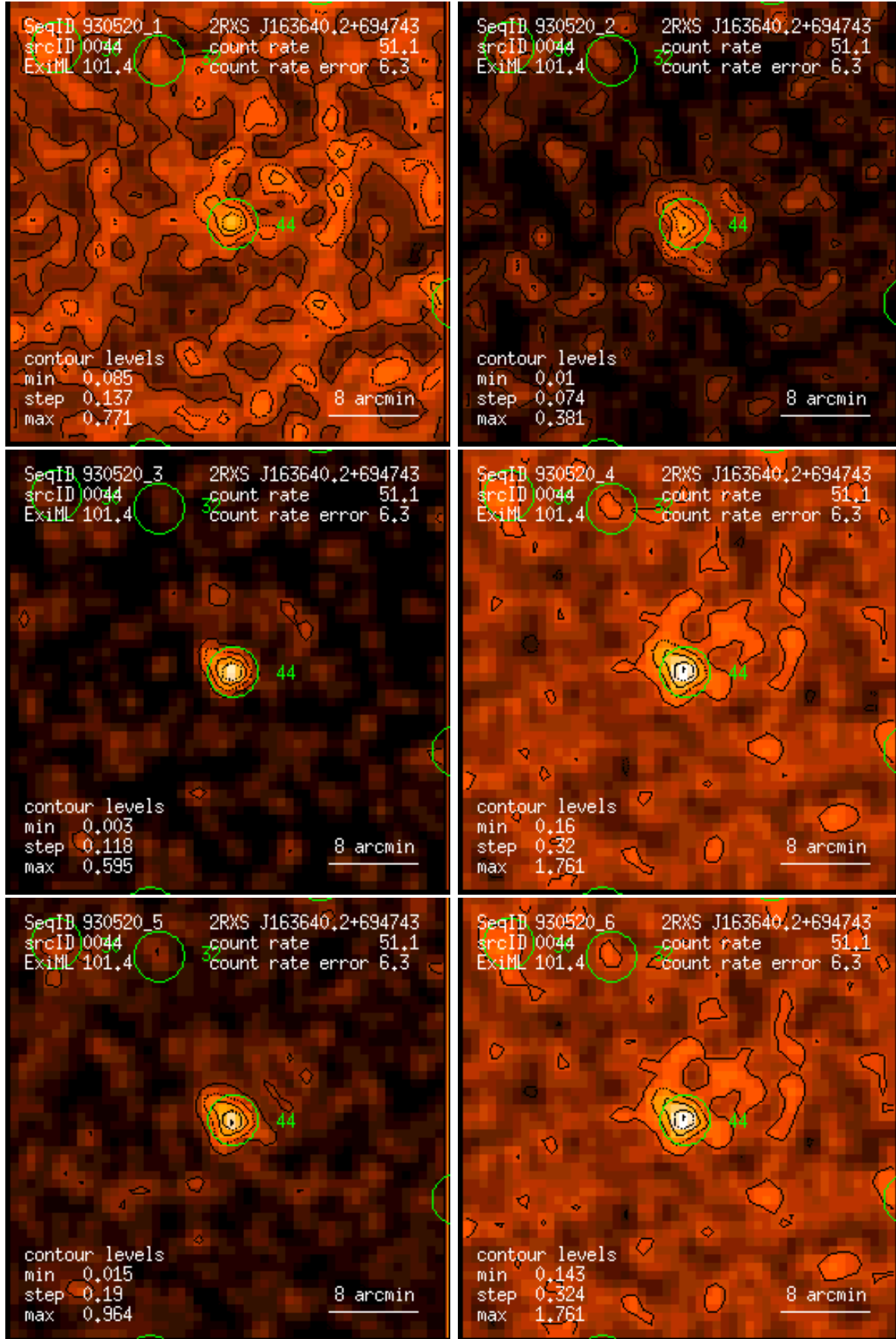
Figure 44: RASS 930520: detection 0044: band rate images, Gaussian filter: (1) PSPC channels 11 – 41, (2) 52 – 90, (3) 91 – 201, (4) 11 – 235, (5) 52 – 201, (6) 11 – 201. Broad band rates in counts/ks. Band rate contour levels in counts/ks/arcmin 2 .
