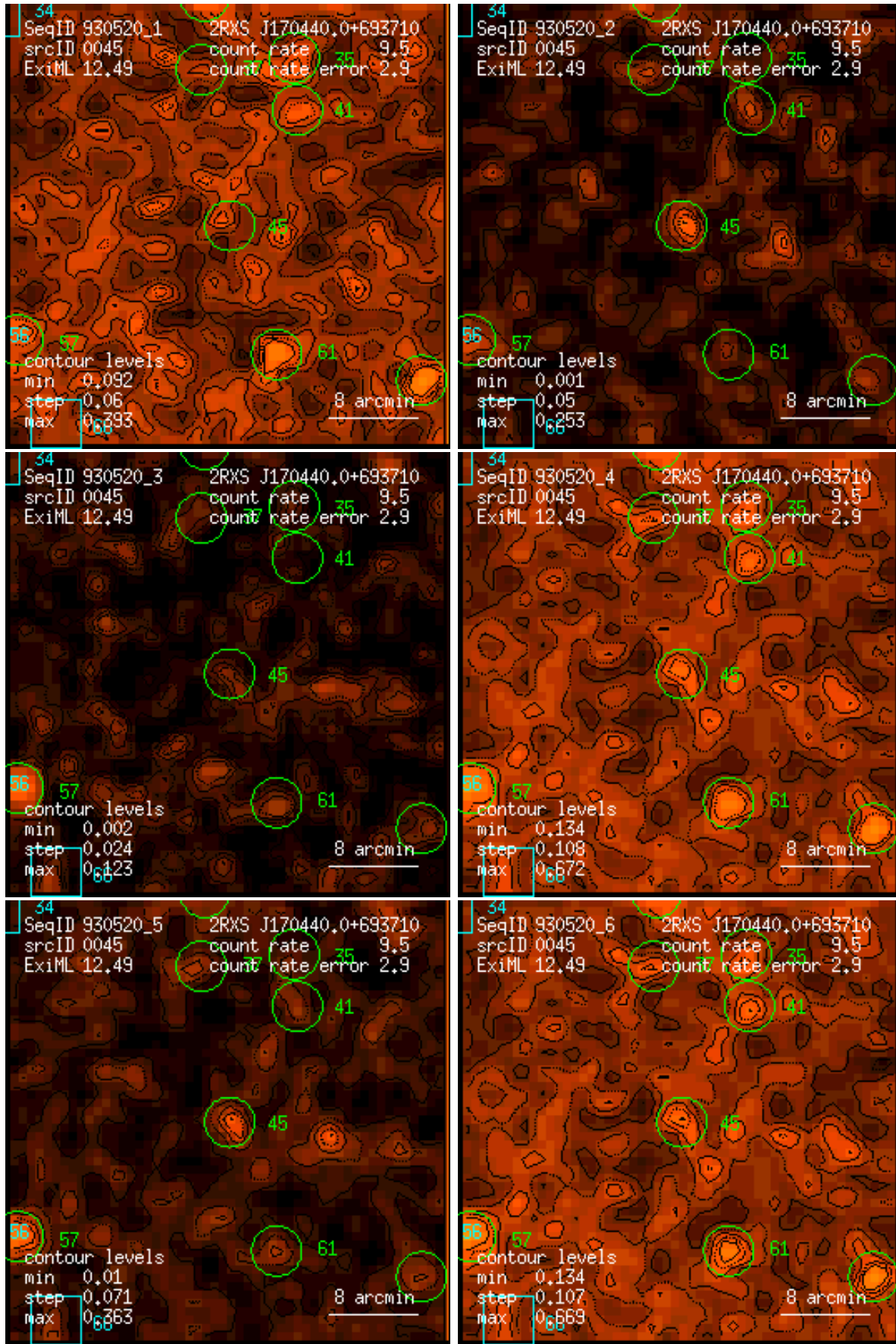
Figure 45: RASS 930520: detection 0045: band rate images, Gaussian filter: (1) PSPC channels 11 – 41, (2) 52 – 90, (3) 91 – 201, (4) 11 – 235, (5) 52 – 201, (6) 11 – 201. Broad band rates in counts/ks. Band rate contour levels in counts/ks/arcmin 2 .
